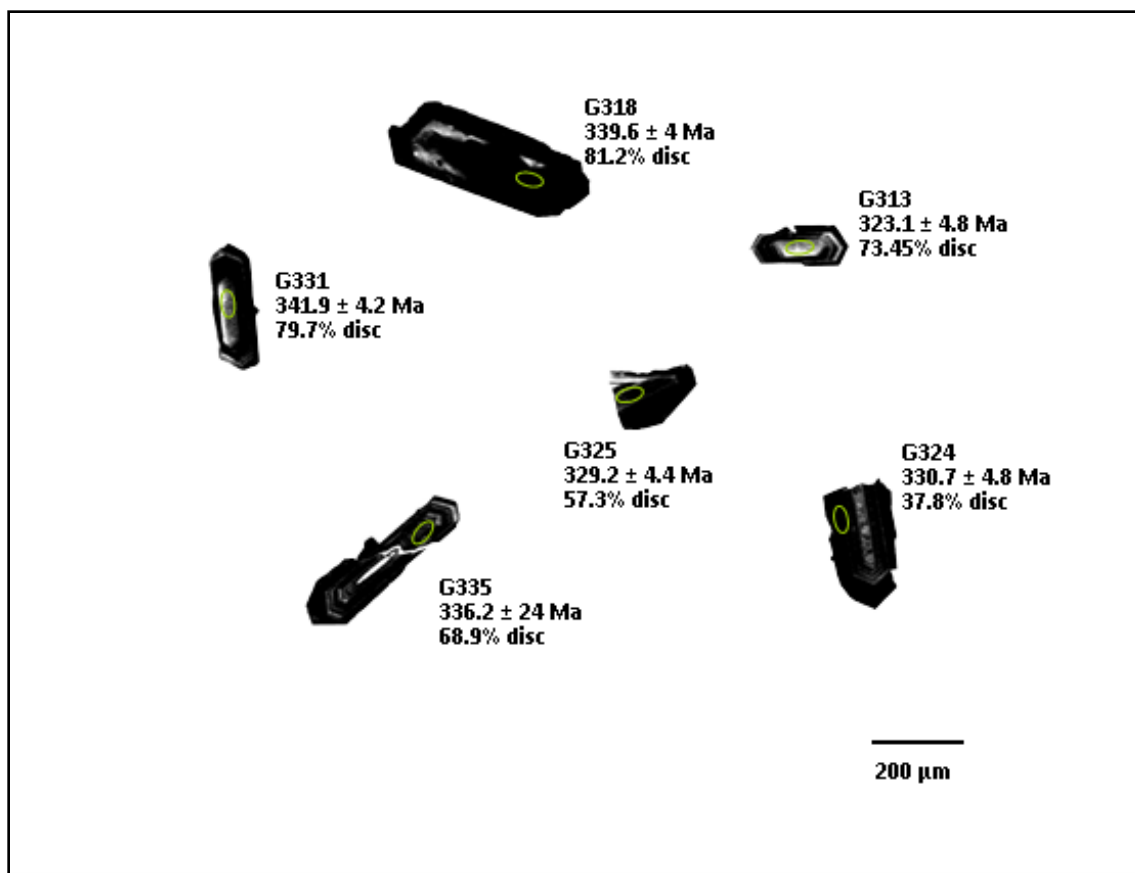
Figure 3: SEM images of typical igneous zircons from the Dartmoor granite of the Cornubian Batholith and resulting data. Ellipses indicate analytical locations and % disc indicates discordance at > 10\% .
