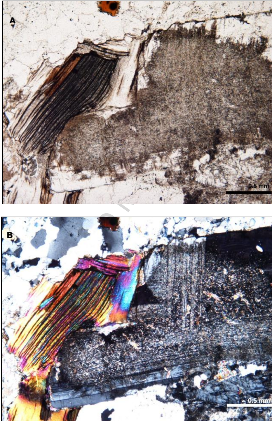
Figure 6: Thin section photos of the Bodmin Moor granite at 4x magnification. Note the dark area of radiation damage within the biotite at the top of the pictures. A) Plane-polarized light. B) Cross-polarized light.
