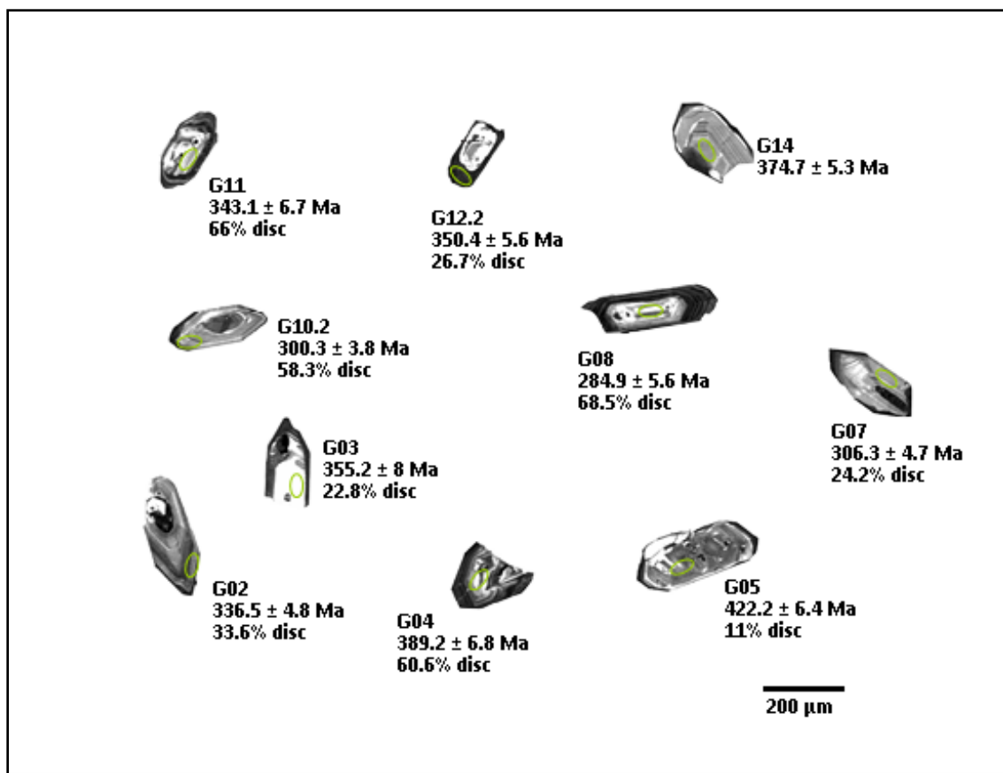
Figure 17: SEM images of typical igneous zircons from the Carnmenellis granite of the Cornubian Batholith and resulting data. Ellipses indicate analytical locations and % disc indicates discordance at > 10\% .
