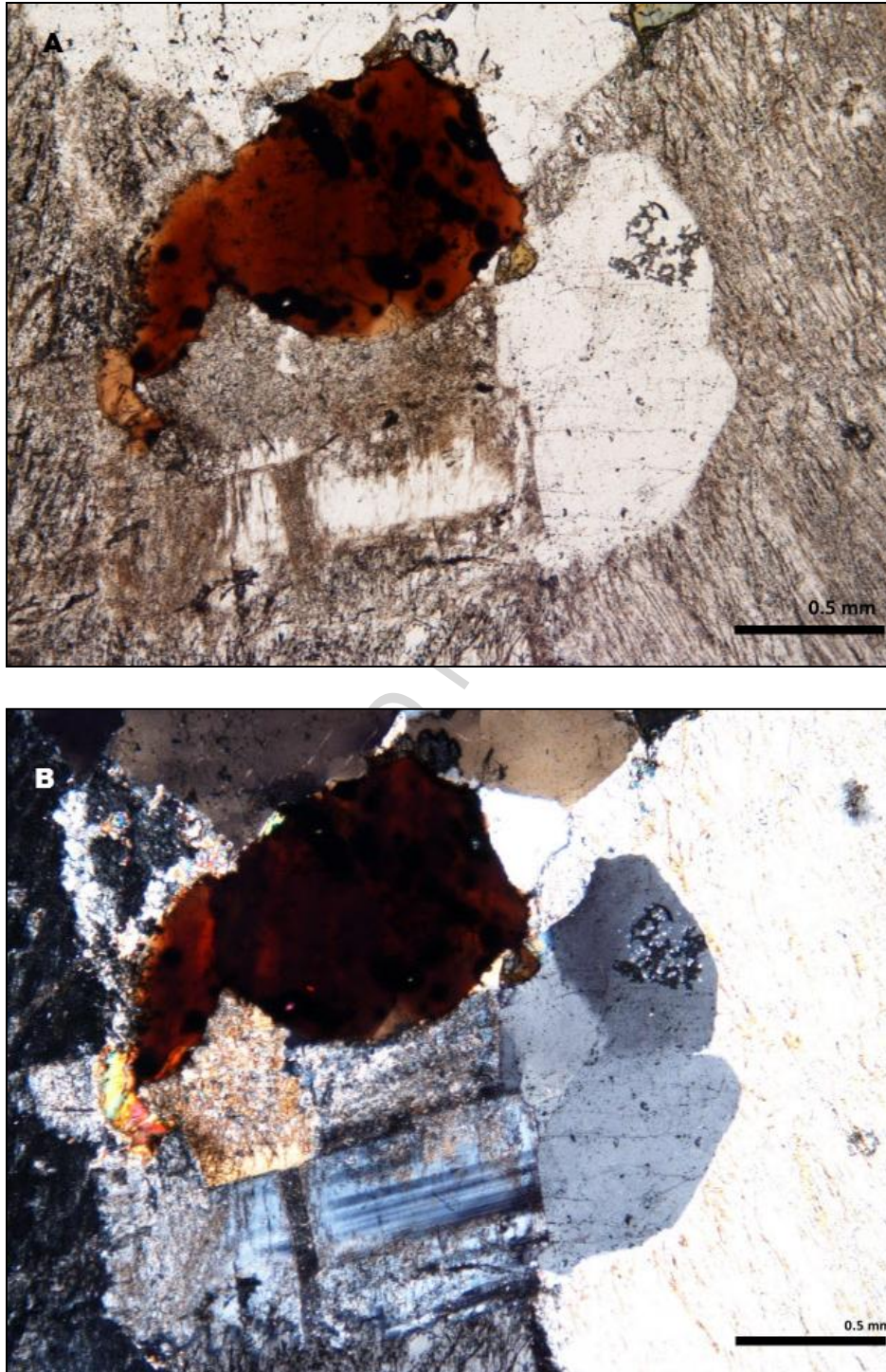
Figure 2: Thin section photos of the Dartmoor granite at 4x magnification. Notice the dark areas of radiation damage within the biotite. A) Plane-polarized light. B) Cross-polarized light.
