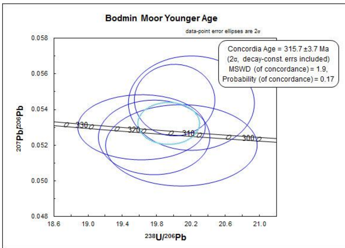
Figure 9: Tera Wasserburg plot of the younger igneous zircon ages from the Bodmin Moor granite of the Cornubian Batholith.
