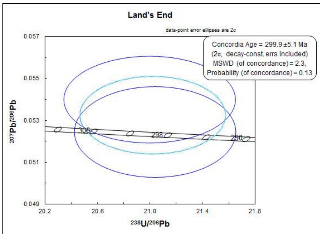
Figure 23: Tera Wasserburg plot of igneous zircon ages from the Land's End granite of the Cornubian Batholith.
