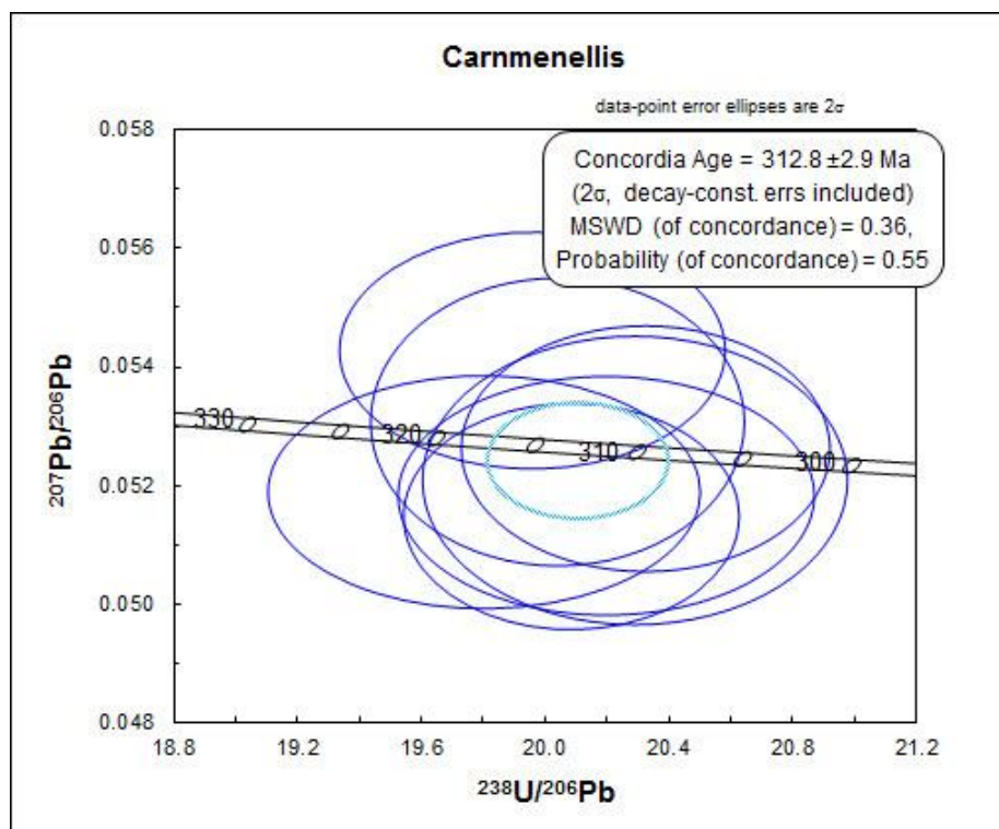
Figure 18: Tera Wasserburg plot of igneous zircon ages from the Carnmenellis granite of the Cornubian Batholith.
