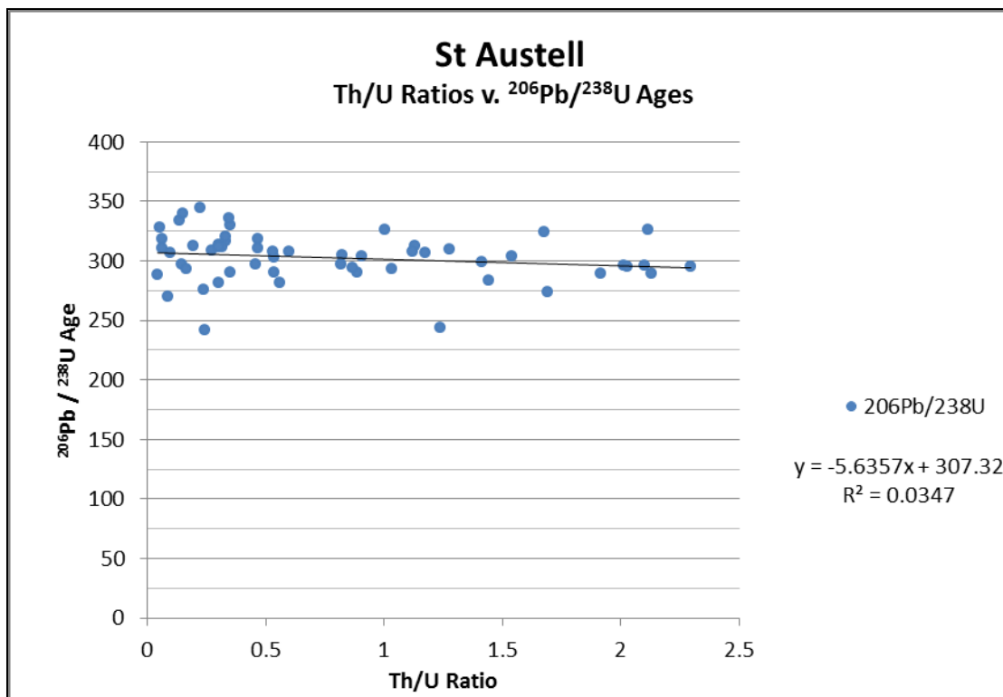
Figure 15: Scatter plot of Th/U ratios vs. ^{206}\text{Pb}/^{238}\text{U} Ages for the St Austell granite.
