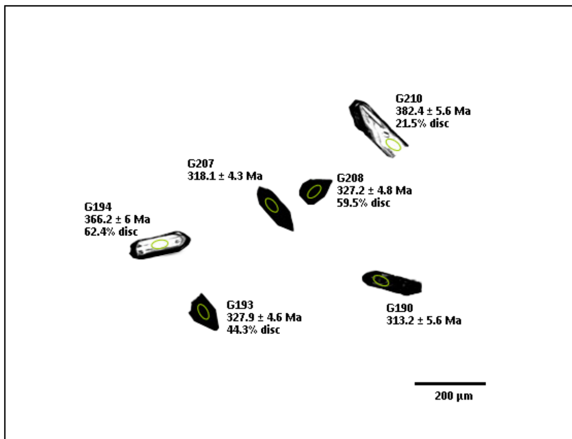
Figure 7: SEM images of typical igneous zircons from the Bodmin Moor granite of the Cornubian Batholith and resulting data. Ellipses indicate analytical locations and % disc indicates discordance at > 10%.
