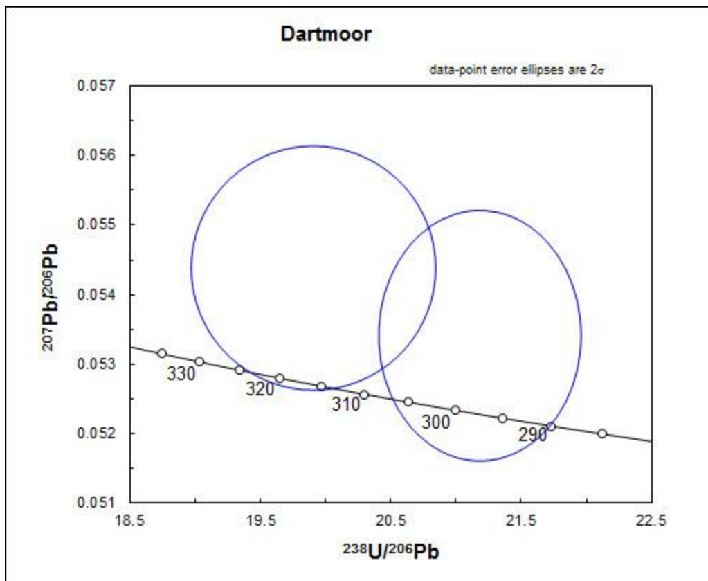
Figure 4: Tera Wasserburg plot of igneous zircon ages from the Dartmoor granite of the Cornubian Batholith.
