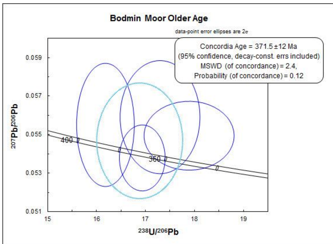
Figure 8: Tera Wasserburg plot of the older (inherited) igneous zircon ages from the Bodmin Moor granite of the Cornubian Batholith.
