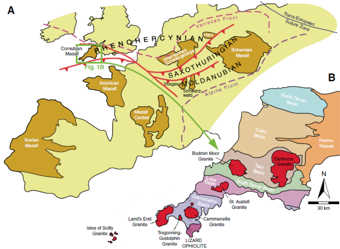
Figure 1: Modified from Pownall et al. (2012). Geological setting of the Cornubian granites within the European Variscides. (A) The Variscan belt of Europe during the Early Carboniferous, modified from Matte (1986) and Franke (1989). (B) Map of the Cornubian granites in the Western Rhenohercynian of SW England, after Shail and Leveridge (2009).
