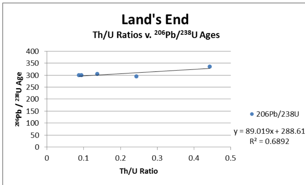
Figure 24: Scatter plot of Th/U ratios vs. ^{206}\text{Pb}/^{238}\text{U} Ages for the Land's End granite.
