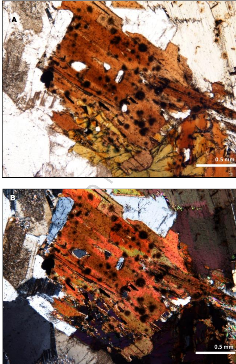
Figure 12: Thin section photos of the St Austell granite at 4x magnification. Notice the dark areas of radiation damage within the biotite. A) Plane-polarized light. B) Cross-polarized light.
