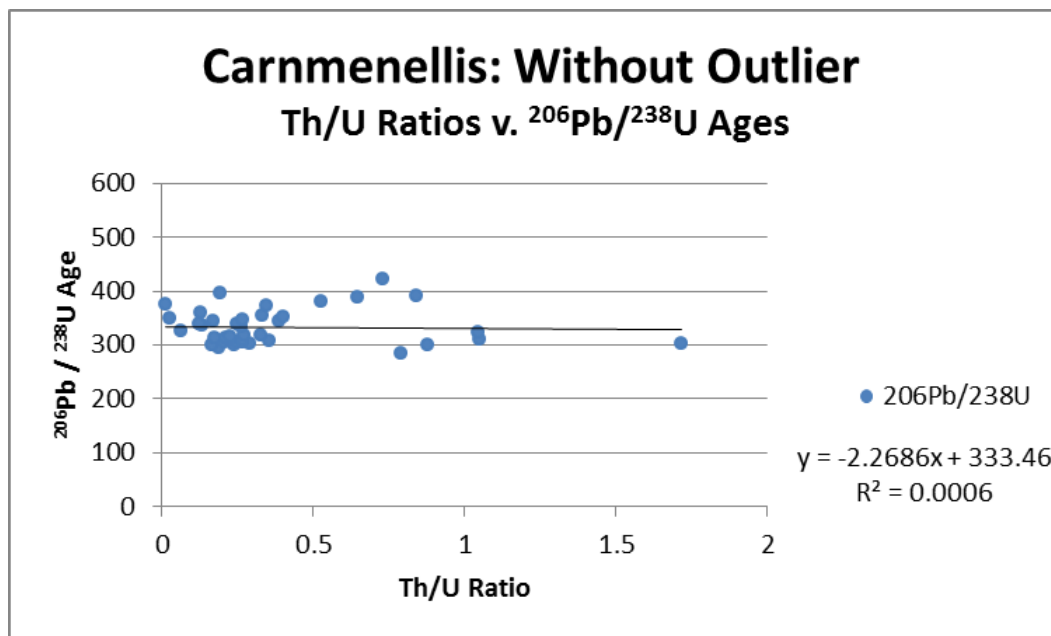
Figure 20: Scatter plot of Th/U ratios vs. ^{206}\text{Pb}/^{238}\text{U} Ages for the Carmmenellis granite with inherited ages excluded.
