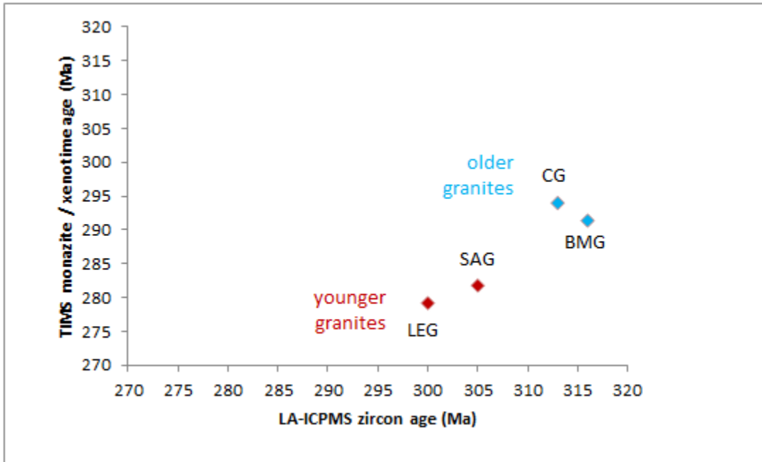
Figure 26: Comparison of LA-ICPMS U–Pb zircon ages (this study) with those from TMS U–Pb monazite / xenotime (Chesley et al., 1993; Chen et al., 1993).
