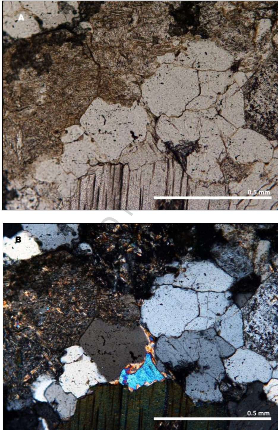
Figure 21: Thin section photos of the Land's End granite at 10x magnification. No halos of radiation damage or zircons were visible, represented by the halo-free biotite in the bottom center. A) Plane-polarized light. B) Cross-polarized light.
