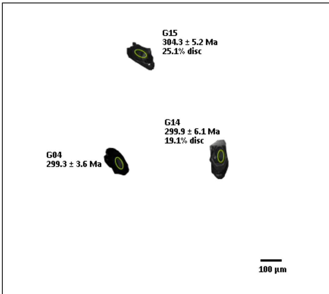
Figure 22: SEM images of typical igneous zircons from the Land's End granite of the Cornubian Batholith and resulting data. Ellipses indicate analytical locations and % disc indicates discordance at > 10%.
