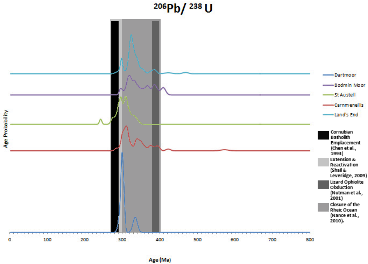
Figure 25: Age distribution plot for each of the five major plutons of the Cornubian Batholith shown in relations to the major tectonic and structural events related to its emplacement.
