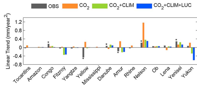
Figure 11. Discharge trends ( \text{mm}/\text{year}^2 ) estimated by DGVMs for 15 river basin regions from 1981 to 2010. DGVM scenario simulations include “CO 2 ” (S1), “CO 2 +CLIM” (S2), and “CO 2 +CLIM+LUC” (S3). * Statistical significance at the 95% ( P < 0.05 ) level. The trend for each model scenario was calculated as the median value of the trends estimated by different DGVM. (The modeled discharge data are unavailable in the Mackenzie Basin under S1 simulation.)
