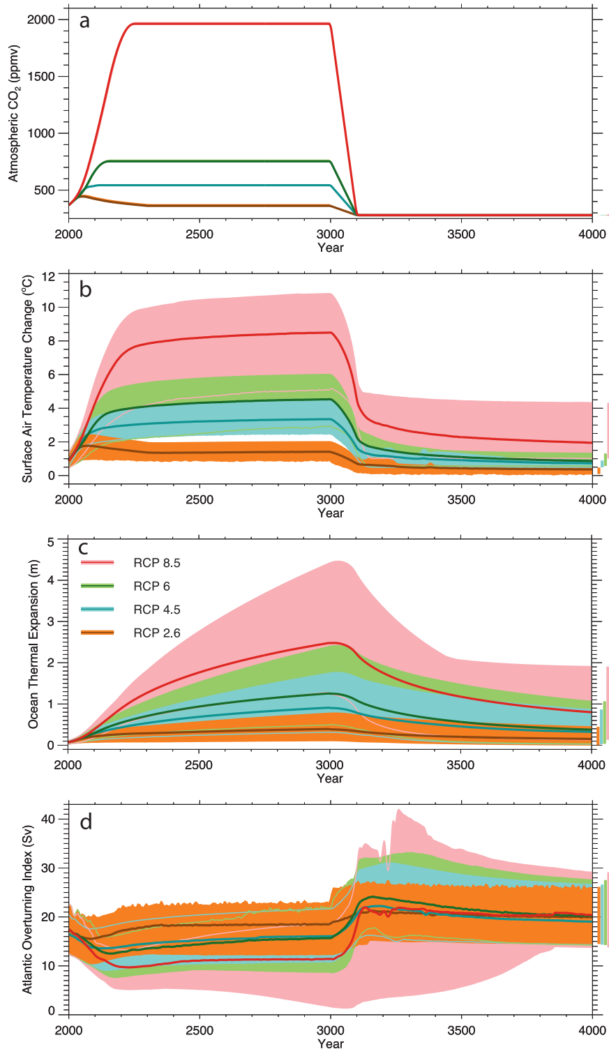
FIG. 11. Time evolution of climate variables for REa simulations with atmospheric \text{CO}_2 after year 3000 decreasing to preindustrial levels over 100 yr: (a) atmospheric \text{CO}_2 , (b) surface air temperature change, (c) ocean thermal expansion, and (d) Atlantic overturning index (maximum of the overturning streamfunction in the North Atlantic). Anomalies in (b) and (c) are relative to preindustrial (1851–60). Shown are the model ensemble averages (thick solid lines), the ranges spanned by all models (shaded domains, delimited by thin solid lines), and the range in the year 3000 (vertical bars on side). Data were smoothed using a 10-yr moving average.
