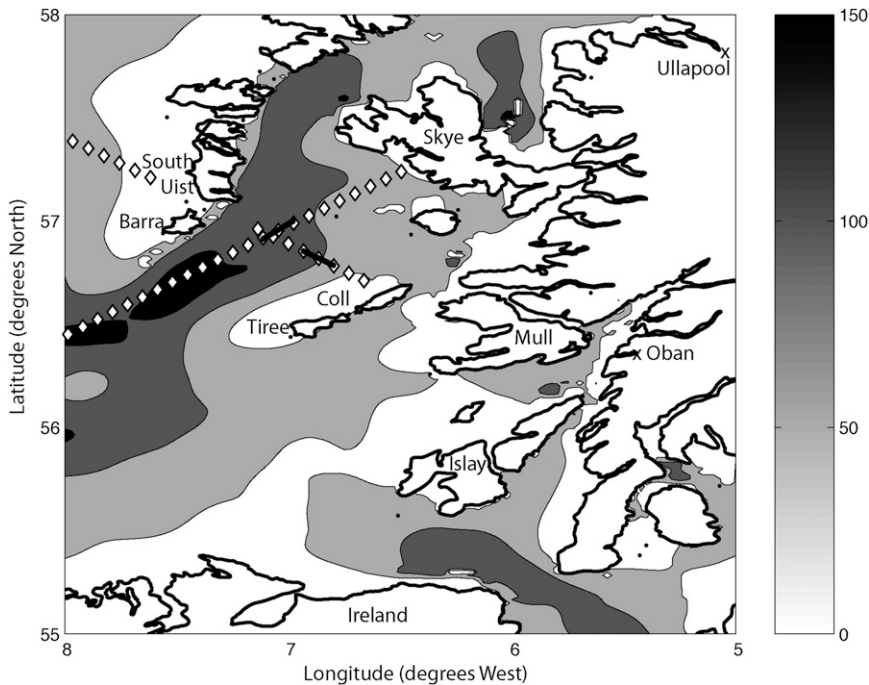
FIG. 5. Map of the region, indicating the two satellite altimeter tracks (denoted by the diamonds) used for wave-height analysis within the Sea of the Hebrides and the surrounding bathymetry (contoured in multiples of 50 m, with darker shading corresponding to successively deeper water).
