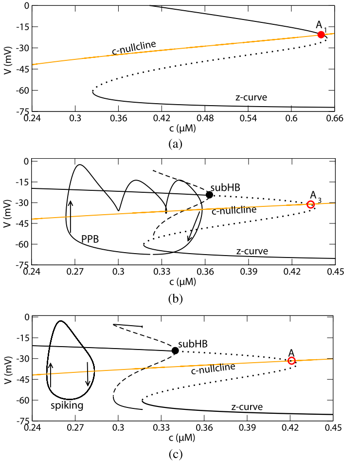
Fig. 13 Two-fast/one-slow analysis for g_{BK} = 0.4 nS, C_m = 10 pF and different values of g_K . The black “z-curve” is the curve of equilibria of the V - n fast subsystem. This has stable (solid) and unstable (dashed) branches. (a) g_K = 0.1 nS, the full system with stable equilibrium ( A_1 ) is in a depolarized steady state. (b) g_K = 4 nS, the fast subsystem has an unstable limit cycle that emerges from the subcritical Hopf bifurcation (subHB). Pseudo-plateau bursting (PPB, black trajectory) is produced. The equilibrium of the full system ( A_3 ) is unstable. (c) g_K = 5.1 nS, the full system produces periodic spiking that appears unrelated to the fast subsystem bifurcation structure. The equilibrium point of the full system ( A ) is unstable. In all panels the system is bistable over a range of c -values. The points A_1 and A_3 are the same equilibrium points as A_1 and A_3 in Fig. 5, respectively.
