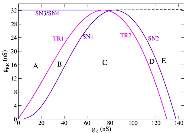
Fig. 7 Two-parameter bifurcation structure for the desingularized system. The curves TR1 and TR2 represent the transcritical bifurcations (type II folded saddle-nodes). The curves SN1-SN4 represent saddle-node bifurcations (type I folded saddle-nodes). The horizontal line is where the fold curves L^+ and L^- coalesce. A codimension-2 bifurcation occurs at the intersection of the SN curves.
