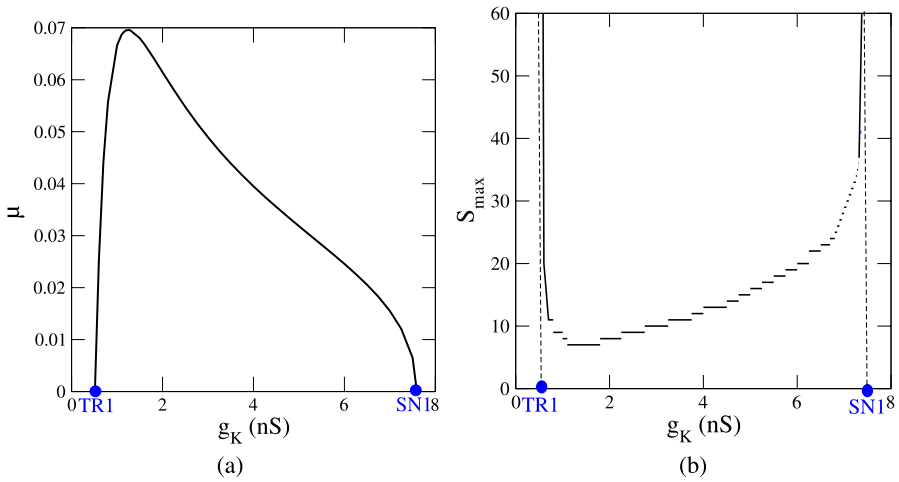
Fig. 8 The effects of varying g_K on the eigenvalue ratio ( \mu ) and the maximum number of oscillations ( S_{max} ) for g_{BK} = 0.4 nS. (a) \mu = 0 at TR1 and SN1. (b) S_{max} is largest near the bifurcation points.
