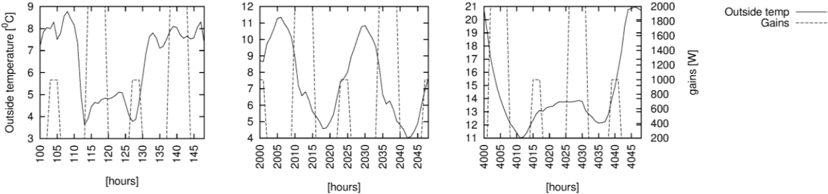
Figure 8 - Inputs of the dynamic models. Outside temperature and heat flow for three 48 hours periods in winter, spring and summer.
