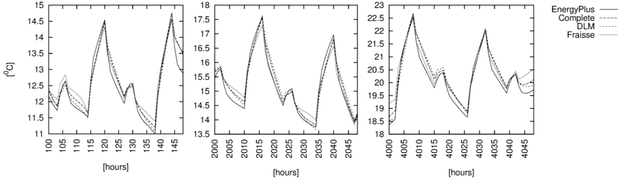
Figure 9 - Temporal response for the model when using that use the construction "Light".
