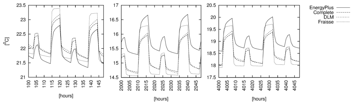
Figure 13 - Temporal response for the model when using construction "Proof".
