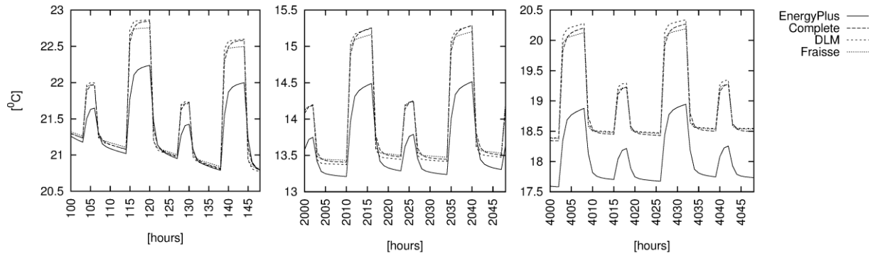
Figure 10 - Temporal response for the model when using construction "Heavy".
