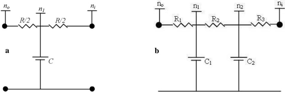
Figure 1 - a) Two-port electric equivalent of a single material layer. b) "3R2C" LPM.
