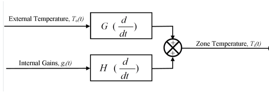
Figure 4. Internal temperature as the sum of the response of two linear systems.
