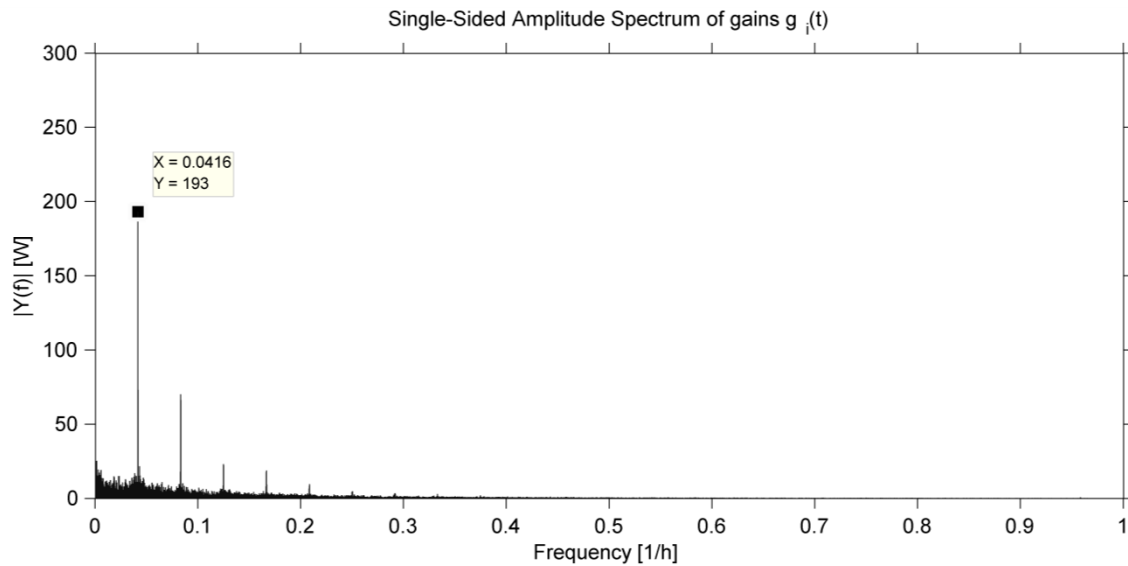
Figure 3 - Representation of the harmonics of a time series of internal gains in a building simulation (1 year) from data sampled at a resolution of 1 minute. Note the peak representing the harmonic with the largest amplitude with a 24 hour period.
