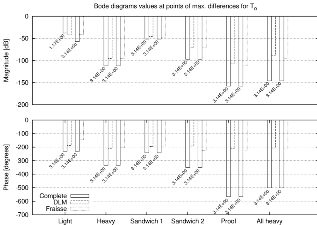
Figure 6 - Values of magnitude and phase for the three models when using T_o as input. The pairs of bars show the value of the Bode diagram for the complete and the reduce model (DLM or Fraise's) and the angular frequency at which the maximum difference is found (the angular frequency is in rad/hour).
