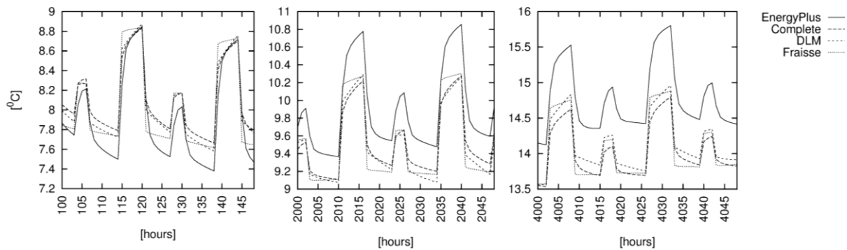
Figure 14 - Temporal response for the model when using construction "All heavy".
