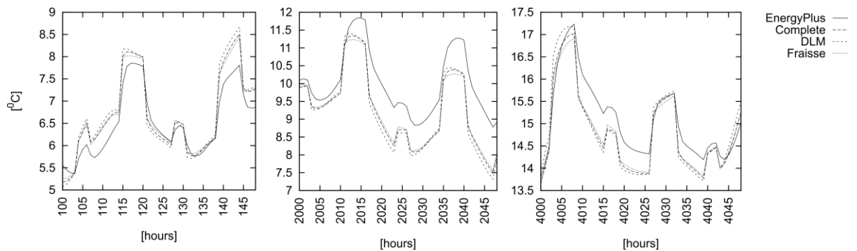
Figure 11 - Temporal response for the model when using construction "Sandwich 1".
