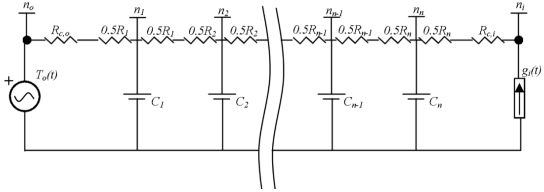
Figure 2 - RC network representing a construction with n layers subjected to a time-varying outside temperature, T_o(t) , and time-varying internal gains, g_i(t) . Note: the voltage source has been represented as sinusoidal, but it should be considered as a time series.
