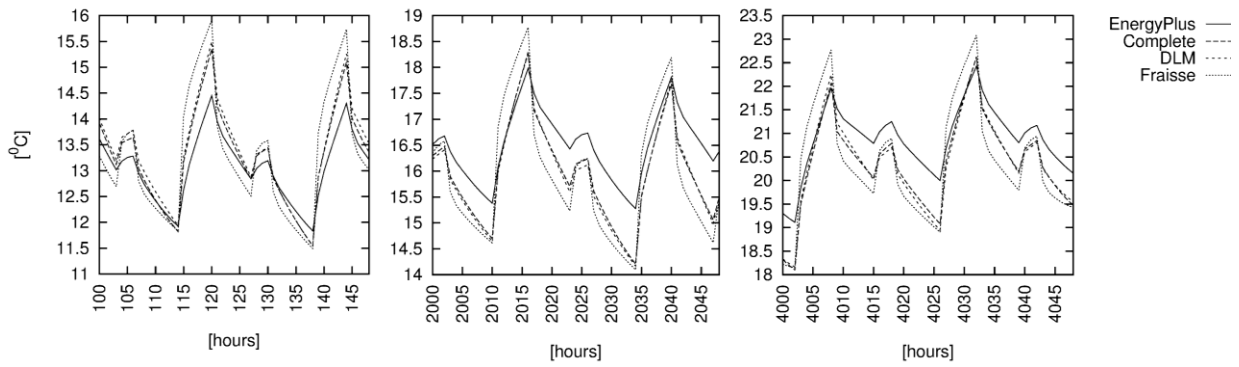
Figure 12 - Temporal response for the model when using construction "Sandwich 2".
