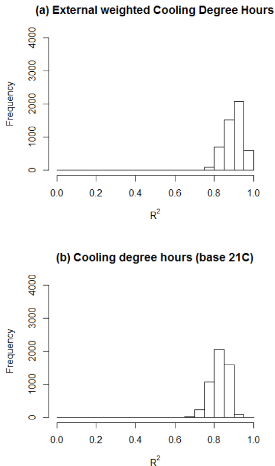
Figure 3: Histogram of the r^2 values for linear regression for internal WCDH against (a) external WCDH and (b) CDH (base temperature of 21 °C).
