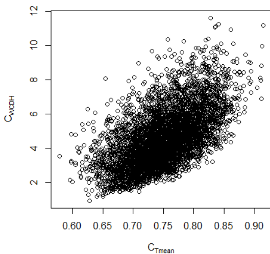
Figure 5: C_{WCDH} against C_{Tmean} for all 5000 building.
