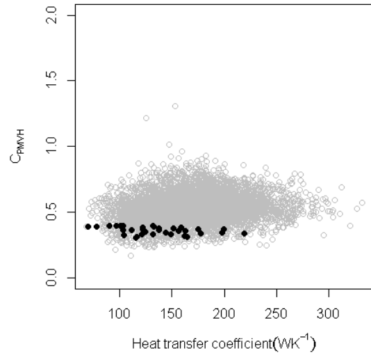
Figure 8: C_{PMVH} against the total heat transfer coefficient. The 33 optimal buildings in terms of minimizing C_{WCDH} and C_{PMVH} are shown by dark circles
