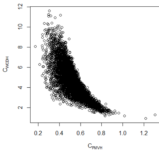
Figure 6: C_{WCDH} against C_{PMVH} for all 5000 buildings
