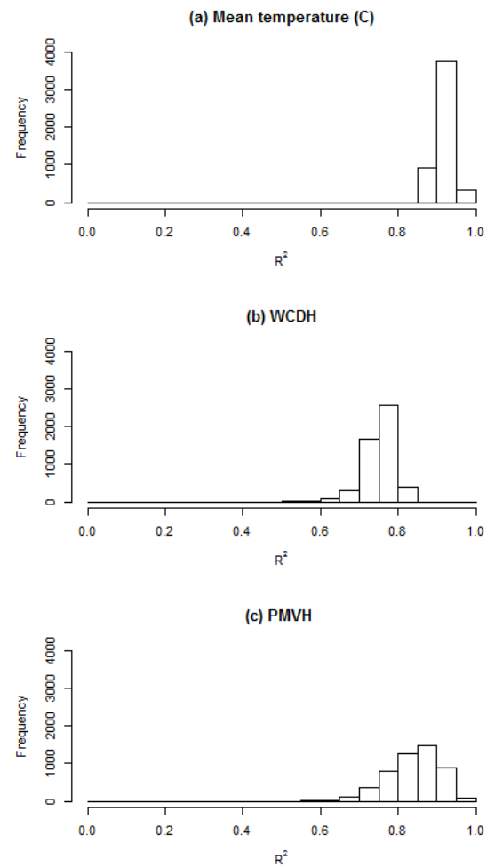
Figure 2: Histogram of the r^2 values for linear regression for (a) internal mean summer temperature, (b) internal WCDH and (c) internal PMVH against the external mean summer temperature
