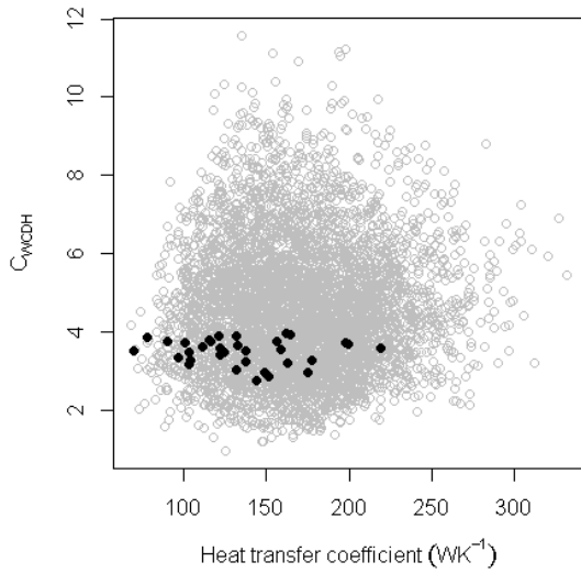
Figure 7: C_{WCDH} against the total heat transfer coefficient. The 33 optimal buildings in terms of minimizing C_{WCDH} and C_{PMVH} are shown by dark circles
