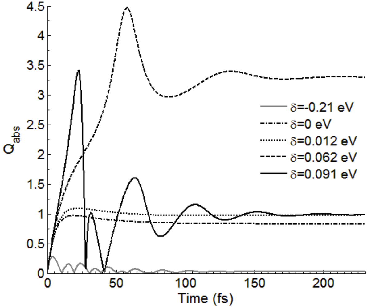
Figure 4. Calculated Q_{abs}(t, \omega) for a 100 nm diameter nanosphere of 3.22% TDDBC:PVA warming up a pure state at t = 0 with a 1 mW laser set at five different detunings \delta from the exciton transition.
