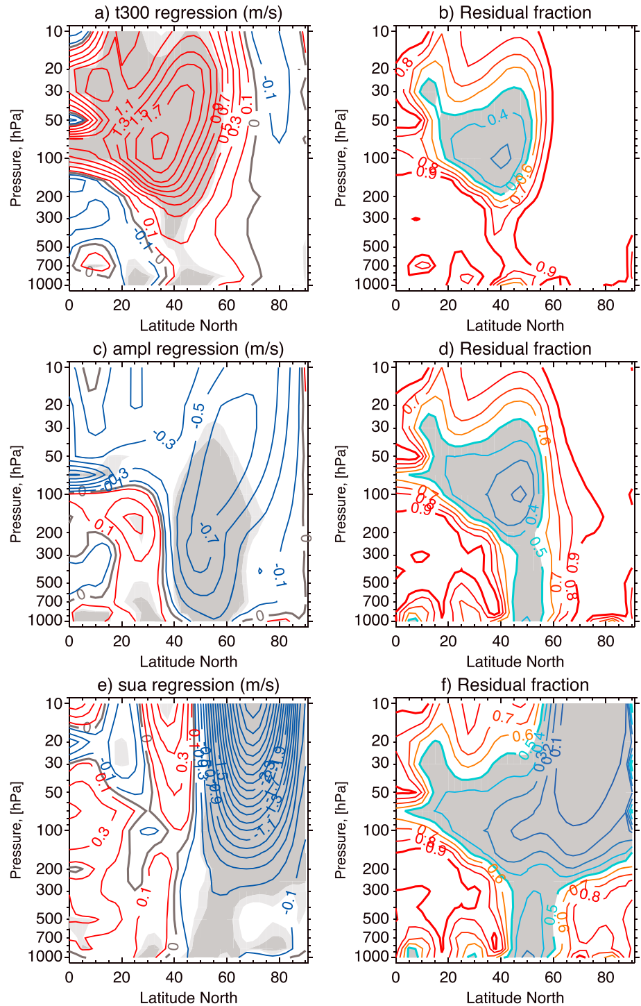
Figure 4. CMIP5 multimodel ensemble, DJF zonally averaged zonal wind change (2061–2100 RCP8.5 minus 1961–2000 historical). Regression coefficients (contours: 0, \pm 0.1 , and every 0.2 m s^{-1} thereafter) for (a) \Delta T300 , (c) \Delta AMPL , and (e) \Delta SUA . Ratio (contours: 0.1) between the intermodel variance from residuals and that from the total fields, with the residual fields respectively from (b) \Delta T300 , (d) \Delta AMPL , and (f) \Delta SUA regressions. In Figures 4a, 4c, and 4e, dark (light) shadings mark areas where the slope of the regression is significantly different from zero according to two-tailed t test with p < 0.05 ( < 0.1 ). In Figures 4b, 4d, and 4f, gray shading indicates ratios less than 0.5.
