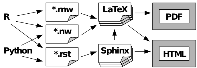
Fig. 1: Summary of the possible workflows using lpEdit. First, a language, either R or Python is selected then it is embedded into a specific document (*.rnw, *.nw or *.rst). Next a LaTeX or Sphinx project is built for the document, which then allows for both HTML and PDF output formats.
