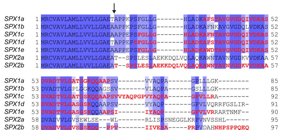
Fig 2. Amino acid alignment of the highly abundant SPX1a-1e and SPX2a and 2b proteins. Protein sequences were aligned using Muscle v3.7 and the degree of amino acid identity of each residue is represented by dark (strictly identical) to light purple shadings (low identity). The cleavage site of the predicted signal peptide determined using SignalP v4.1 is indicated by an arrow. De novo sequenced peptides obtained after mass spectrometry and used for the identification of these proteins are indicated in red.
