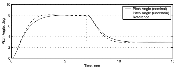
Fig. 1. Closed loop response to step changes in pitch angle
