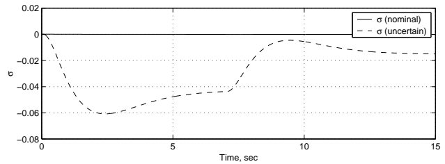
Fig. 2. Deviation from the sliding surface S
