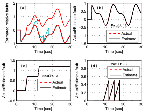
Fig. 3. Fault reconstruction with faults introduced in randomly chosen nodes
