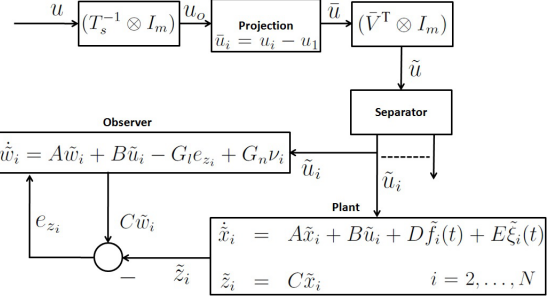
Fig. 1. Observer architecture
