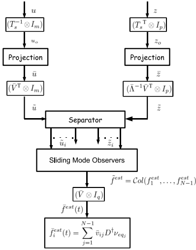
Fig. 2. Fault reconstruction architecture
