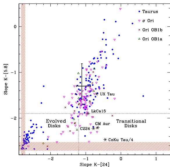
Fig. 3.— Spitzer color-color diagram of objects in different associations and clusters. Observations are shown for populations of different ages: Taurus, 1–2 Myr (Luhman et al. 2010); \sigma Ori, 3 Myr (Hernández et al. 2007a); Ori OB1b, 7 Myr; Ori OB1a, 10 Myr (Hernández et al. 2007b). The hatched region corresponds to stellar photospheric colors. The error bars represent the median and quartiles of Taurus objects (i.e., where most full disks are expected to lie). Well characterized transitional disks (GM Aur, CoKu Tau/4, CVSO224; Espaillat et al. 2008a) and pre-transitional disks (LkCa 15, UX Tau) are indicated with asterisks. The dotted lines correspond to the lower quartile of disk emission in \sigma Ori, and roughly separate the evolved disks (lower left) from the transitional disks (lower right). Note that the pre-transitional disks do not lie below the dotted line, highlighting that it is harder to identify disk gaps based on colors alone. Figure adapted from Hernández et al. (2007b).
