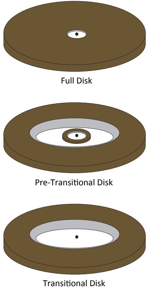
Fig. 2.— Schematic of full (top), pre-transitional (middle), and transitional (bottom) disk structure. For the full disk, progressing outward from the star (black) is the inner disk wall (light gray) and outer disk (dark gray). Pre-transitional disks have an inner disk wall (light gray) and inner disk (dark gray) followed by a disk gap (white), then the outer disk wall (light gray) and outer disk (dark gray). The transitional disk has an inner disk hole (white) followed by an outer disk wall (light gray) and outer disk (dark gray).
