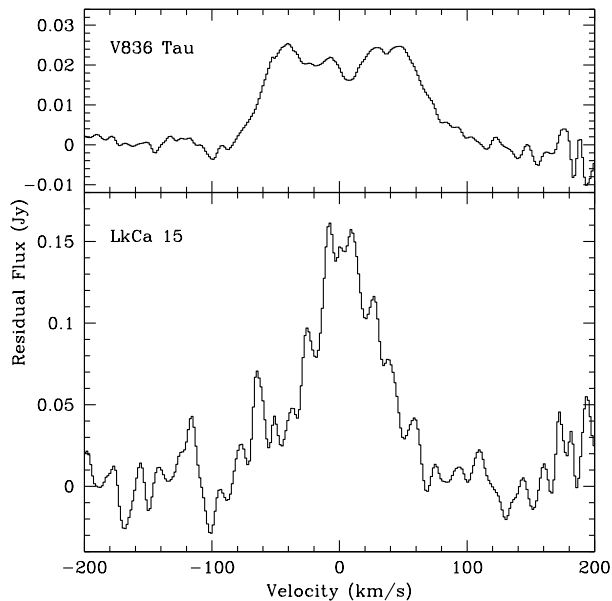
Fig. 8.— Rovibrational line profiles of CO v=1-0 emission from V836 Tau (top) and LkCa 15 (bottom) after correction for stellar CO absorption (Najita et al. 2008). The double-peaked profile of V836 Tau indicates that the gas emission is truncated beyond \sim 0.4 AU. The centrally-peaked LkCa 15 profile indicates gas emission extending to much larger radii.
