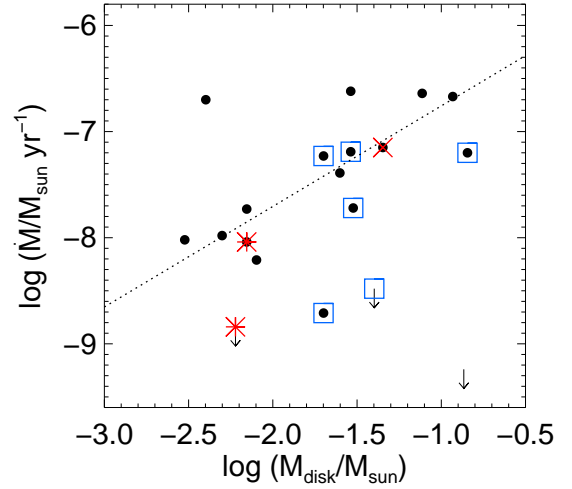
Fig. 12.— Preliminary \dot{M}_* - M_d for disks in Ophiuchus. The dotted line indicates the locus occupied by CTTS in Taurus ( Najita et al. 2007a). Disks with submm cavities and (pre-)transitional disk SEDs are overlaid with a star (SR 21, bottom left; DoAr 44, middle); the disk with a submm cavity but no obvious SED MIR deficit (SR 24S) is overlaid with an “X”. Sources with A_V > 14 ( McClure et al. 2010) are indicated with a blue box. Objects where only upper limits were available for the accretion rates are indicated with an arrow (including SR 21, GSS 26, DoAr 25). Accretion rates are from Natta et al. (2006) if available, otherwise from Eisner et al. (2005), and Valenti et al. (1993) (scaled). Disk masses are from Andrews and Williams (2007); Andrews et al. (2010).
