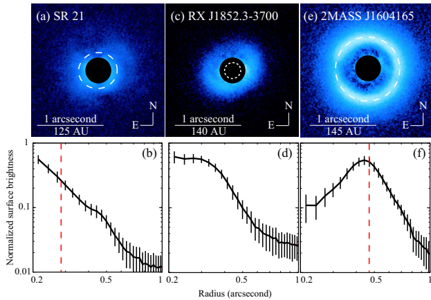
Fig. 5.— NIR polarimetric images of transitional disks in the H band (top; 1.6 \mu\text{m} ) along with their averaged radial surface brightness profiles along the major disk axis (bottom). Broken lines in the top and bottom panels correspond to the radius of the outer wall as measured with submm imaging and/or SEDs. We note that the regions of the inner disk that cannot be resolved are masked out in the panels. From left to right the objects are as follows: SR 21 (Follette et al. 2013), RX J1852–3700 (Kudo et al., in prep.), RX J1604–2130 (Mayama et al. 2012).
