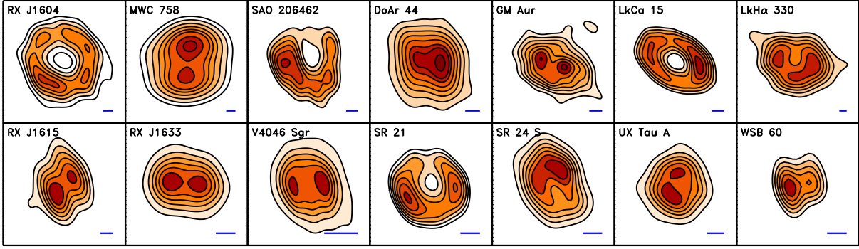
Fig. 4.— A gallery of 880 \mu\text{m} dust continuum images from the Submillimeter Array for (pre-)transitional disks in nearby star-forming regions. From left to right, the panels show the disks around RX J1604.3–2130 ( Mathews et al. 2012 ), MWC 758 ( Isella et al. 2010b ), SAO 206462 ( Brown et al. 2009 ), DoAr 44 ( Andrews et al. 2009 ), GM Aur ( Hughes et al. 2009 ), LkCa 15 ( Andrews et al. 2011b ), LkHa 330 ( Brown et al. 2008 ), RX J1615.3–3255 ( Andrews et al. 2011b ), RX J1633.9–2442 ( Cieza et al. 2012 ), V4046 Sgr ( Rosenfeld et al. 2013 ), SR 21 ( Brown et al. 2009 ), SR 24 S ( Andrews et al. 2010 ), UX Tau A ( Andrews et al. 2011b ), and WSB 60 ( Andrews et al. 2009 ). A projected 30 AU scale bar is shown in blue at the lower right corner of each panel.
