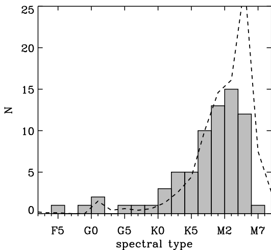
Fig. 13.— The distribution of spectral types for the known transitional disks with spectral type F5 or later. The dashed line indicates the combined parent sample of all disks in the 1–3 Myr old regions, scaled down by a factor of 10, highlighting the apparent deficit of transitional disks around stars later than \sim M4 .
