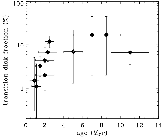
Fig. 11.— The transitional disk fraction for ten star-forming regions and young clusters as a function of mean stellar age. Fractions were estimated by taking the ratio of the number of objects that exhibit a transitional disk SED with the total number of disks in each region. Evolved disks and pre-transitional disks are not included here. The data are taken from (in order of mean age): Arnold et al. (2012a), NGC 1333; McClure et al. (2010), Ophiuchus; Furlan et al. (2011), Taurus; Manoj et al. (2011), Chamaeleon I; Flaherty and Muzerolle (2008), NGC 2068/2071; Oliveira et al. (2010), Serpens; Muench et al. (2007), IC 348; Hernández et al. (2007a), Orion OB1a/b; Megeath et al. (2005), \eta Chamaeleontis association; Luhman and Mamajek (2012), Upper Scorpius association.
