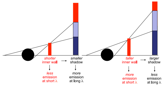
Fig. 7.— Schematic depicting the proposed link between the observed variability and disk structure based on the SED modeling from Fig. 6. Medium gray corresponds to visible areas of the disk wall, while light gray and dark gray areas are in the penumbra and umbra, respectively. The MIR variability observed in pre-transitional disks can be explained by changes in the height of the inner disk wall, which results in variable shadowing of the outer wall.
