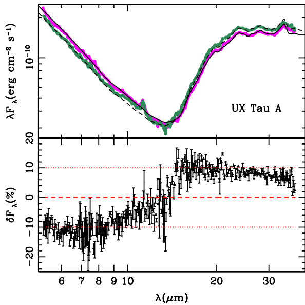
Fig. 6.— Top: Observed Spitzer IRS spectra (gray) and models (solid and broken black lines) for the pre-transitional disk of UX Tau A. The variability between the two spectra can be reproduced by changing the height of the inner disk wall in the model by 17%. Bottom: Percentage change in flux between the two IRS spectra above. The observed variability cannot be explained by the observational uncertainties of IRS (error bars). Figure adapted from Espaillet et al. (2011) .
