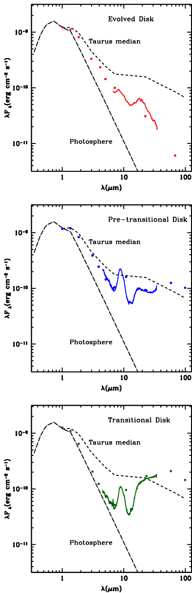
Fig. 1.— SEDs of an evolved disk (top; RECX 11; Ingleby et al. 2011), a pre-transitional disk (middle; LkCa 15; Espaillet et al. 2007), and a transitional disk (bottom; GM Aur; Calvet et al. 2005). The stars are all K3-K5 and the fluxes have been corrected for reddening and scaled to the stellar photosphere (dot-long-dashed line) for comparison. Relative to the Taurus median (short-dashed line; D’Alessio et al. 1999), an evolved disk has less emission at all wavelengths, a pre-transitional disk has a MIR deficit (5–20 \mu\text{m} , ignoring the 10 \mu\text{m} silicate emission feature), but comparable emission in the NIR (1–5 \mu\text{m} ) and at longer wavelengths, and a transitional disk has a deficit of emission in the NIR and MIR with comparable emission at longer wavelengths.
