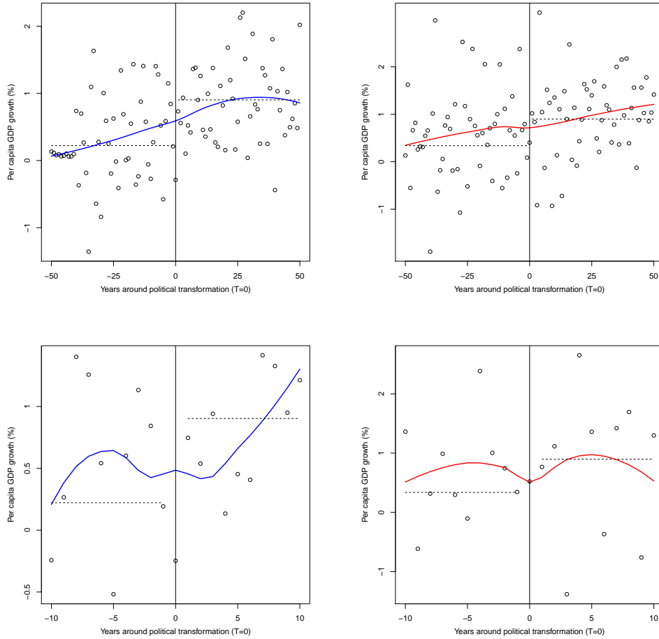
Fig. 1. Time-Demeaned Average Real Per Capita GDP Growth Around Political Transformations
