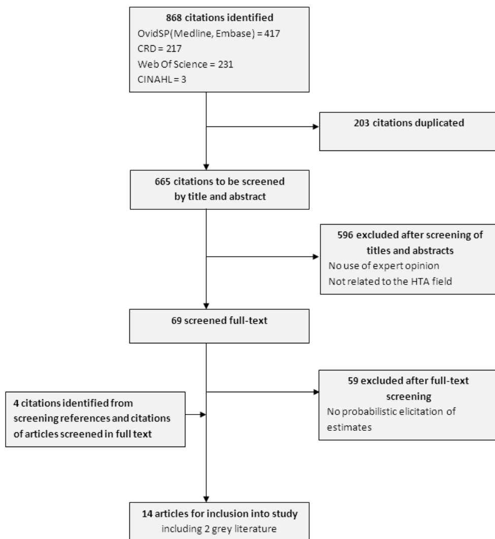
Figure 2. The Flow diagram of search results
