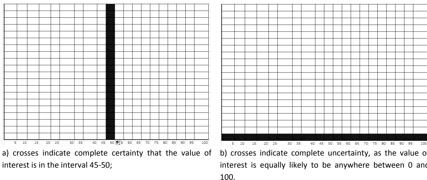
Figure 2. Complete certainty and complete uncertainty represented with the histogram technique.
