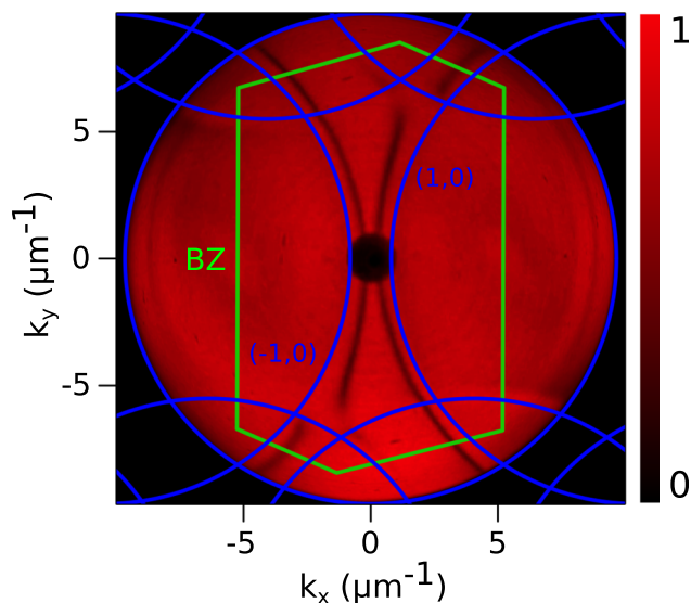
FIG. 2. Experimentally mapped surface plasmon iso-frequency contour via reflectivity (colorscale) at \lambda_0 = 650 nm passing through the first BZ boundary. This contour neither meets the boundary perpendicularly nor is perturbed as it passes through, showing that the group velocity of the SP mode is still finite across the boundary.
