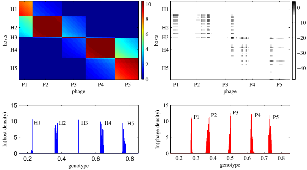
Figure 3: Snapshot of phage-bacteria community structure and interaction during the case study simulation (measured at t = 3.5 \times 10^7 \text{min} ). Upper left : Adsorption rate matrix plot showing pairwise adsorption rate ( \phi\theta_{ij} , values scaled \times 10^{-10} ) for each host ( i ) and phage ( j ) strain present in the current community. Upper right : Infection rate matrix plot showing actual infection rate in the context of the community ( \ln | \phi\theta_{ij} N_i V_j | ) for each host-phage pair. Lower left : Current density of all bacterial genotypes ( \ln | N_i | ). Lower right : Current density of all phage genotypes ( \ln | V_j | ). For ease of reference, labels H1-H5 and P1-P5 are manually attached to identify bacteria and phage “species”.
