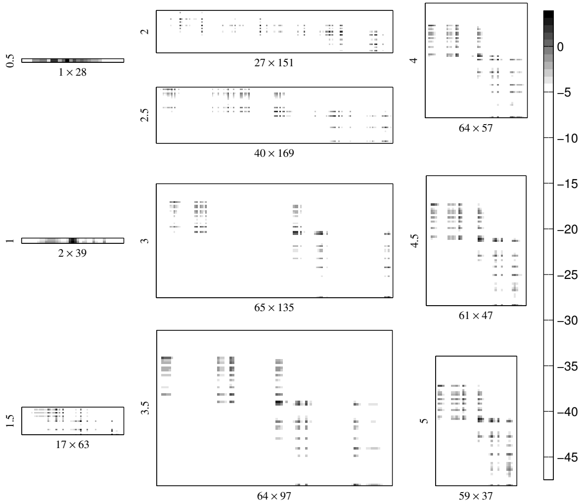
Figure 5: Coevolutionary formation of the infection rate interaction network over time. Grayscale shows pairwise interaction strength ( \ln |\phi\theta_{ij}N_iV_j| ) for bacterial strains (rows) and phage strains (columns). Network size (number of bacterial strains \times number of phage strains) is shown as the x -axis label for each plot, timepoint ( \times 10^7 \text{ min} ) is shown as the y -axis label. Plots show timepoints corresponding to the dotted grid-lines shown in Figure 2, with time increasing down each column, from top-left to bottom-right.
