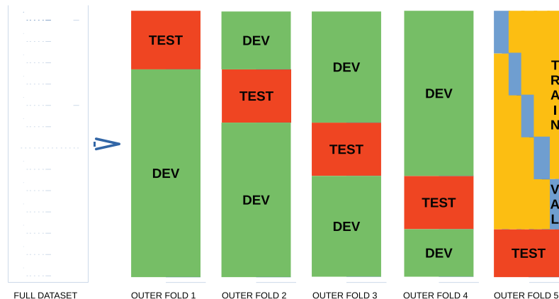
Figure 1 | Schematic representation of the data processing pipeline for hyperparameter tuning and statistical uncertainty estimation.
