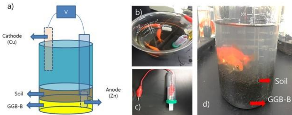
Fig. 2. GGB-B and goldfish treatment a) connection between GGB-B and anode, b) goldfish observation; c) Anode used in experiment d) after three days
