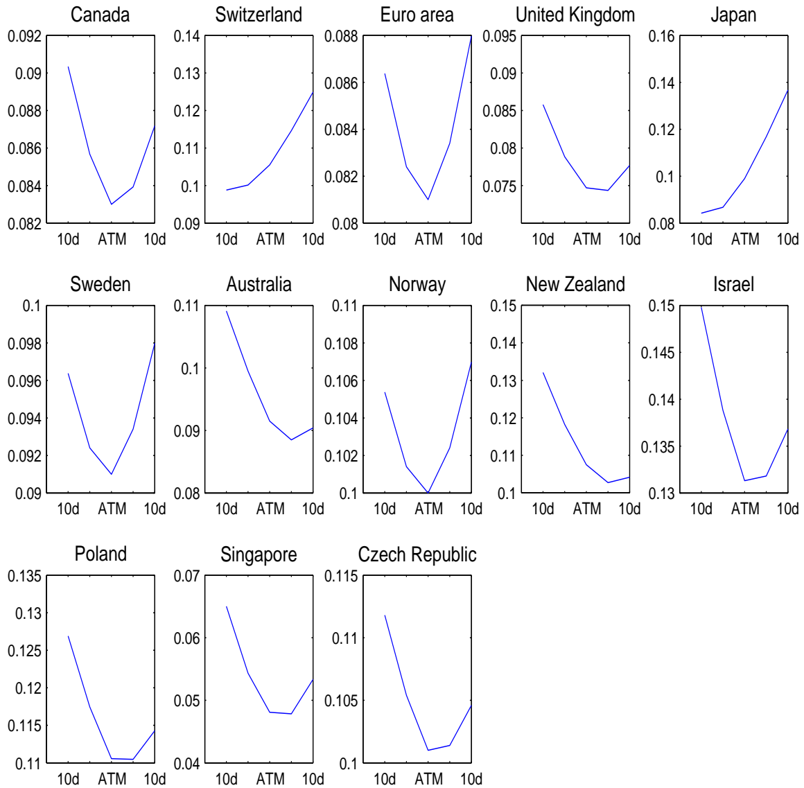
Figure 3: One-Month Option-Implied Volatility Smiles, August 2008
