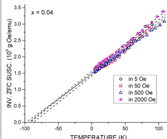
Figure 6. Temperature dependence of the magnetic inverted ZFC susceptibility ( x = 0.04 ) single crystal.
