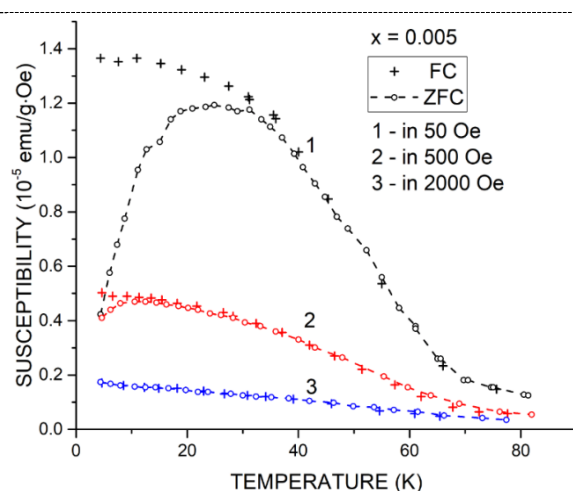
Figure 2. Temperature dependence of the magnetic susceptibility of a ZFA ( x = 0.005 ) single crystal.
