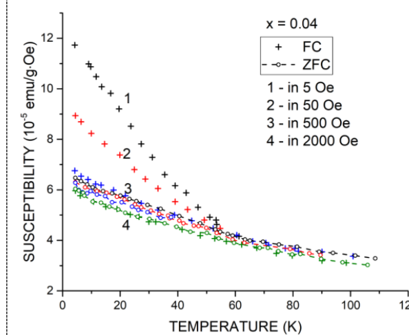
Figure 5. Temperature dependence of the magnetic susceptibility of a ZFA ( x = 0.04 ) single crystal.
