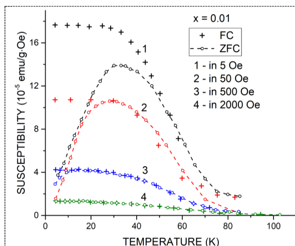
Figure 1. Temperature dependence of the magnetic susceptibility of a ZFA ( x = 0.01 ) single crystal.
