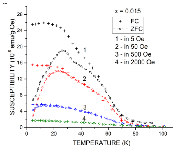
Figure 3. Temperature dependence of the magnetic susceptibility of a ZFA ( x = 0.015 ) single crystal.
