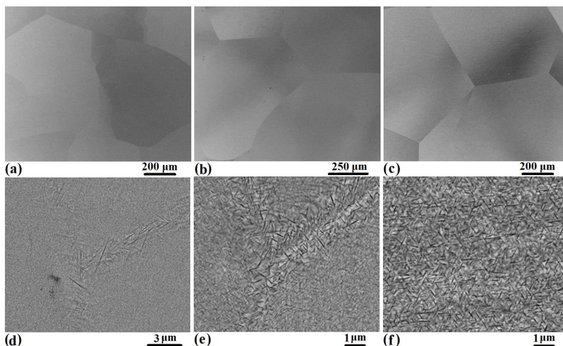
Figure 1. SEM images of the \text{Ti}_{37.5}\text{Nb}_{12.5}\text{Hf}_{25}\text{Al}_{25} (a, d), \text{Ti}_{40}\text{Nb}_{30}\text{Hf}_{15}\text{Al}_{15} (b, e), \text{Ti}_{40}\text{Nb}_{20}\text{Ta}_{10}\text{Hf}_{15}\text{Al}_{15} (c, f) alloys after annealing at 1200 °C, 24 h (a, b, c) and further annealing at 600 °C, 24 h (d, e, f).
