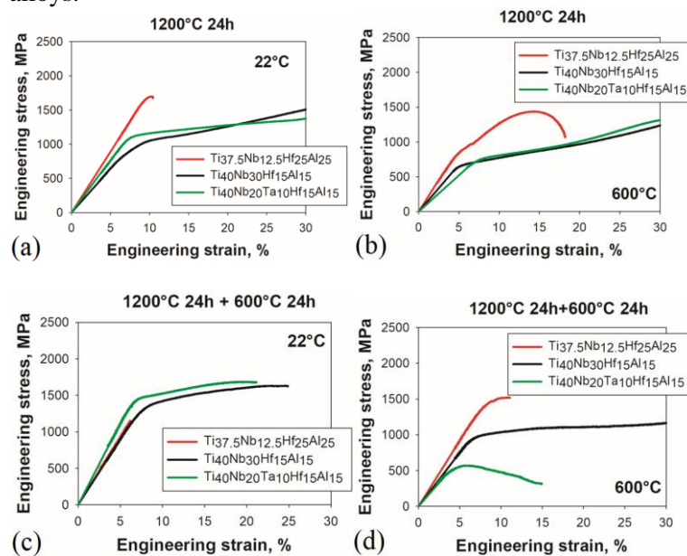
Figure 3. Engineering stress-strain curves of the program alloys after annealing 1200 °C (a, b) and further annealing at 600 °C (c, d) obtained during compression at 22 (a,c) and 600 °C (b,d).
