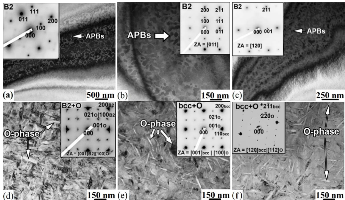
Figure 2. TEM bright-field images of the \text{Ti}_{37.5}\text{Nb}_{12.5}\text{Hf}_{25}\text{Al}_{25} (a, d), \text{Ti}_{40}\text{Nb}_{30}\text{Hf}_{15}\text{Al}_{15} (b, e), \text{Ti}_{40}\text{Nb}_{20}\text{Ta}_{10}\text{Hf}_{15}\text{Al}_{15} (c, f) alloys after annealing at 1200 °C, 24 h (a, b, c) and further annealing at 600 °C, 24h (d, e, f). Selected area electron diffraction patterns used for phase identification are shown in the inserts.
