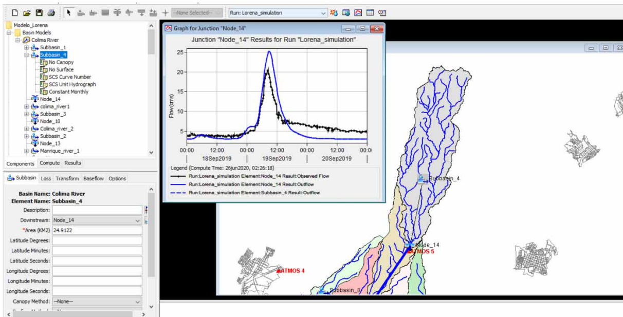
Figure 10 | Simulation of the rainfall-runoff process of the Colima river system (Node 14).
