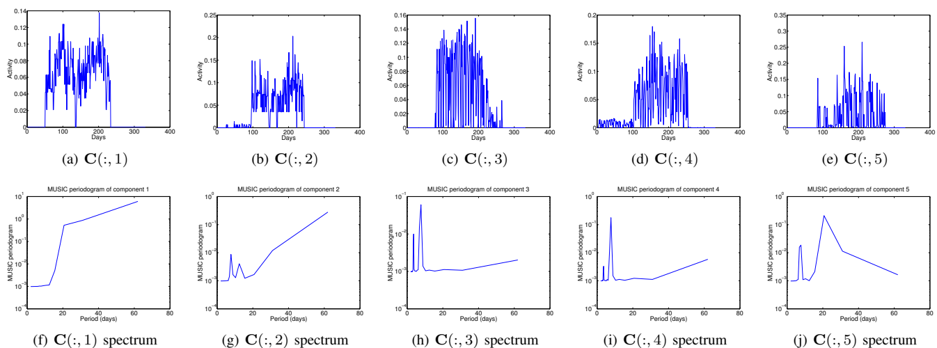
Fig. 2: Temporal profiles and MUSIC spectra for the latent groups of Table I.
