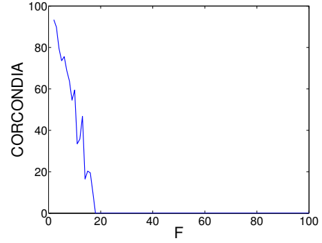
Fig. 1: CORCONDIA values for the Foursquare tensor \underline{\mathbf{T}} as a function of the number of components.
