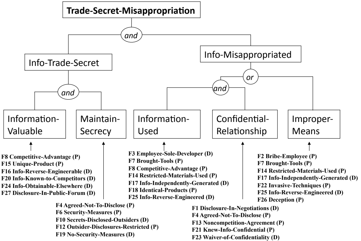
Figure 24: Diagrammatic view of the IBP domain model of issues and associated factors
