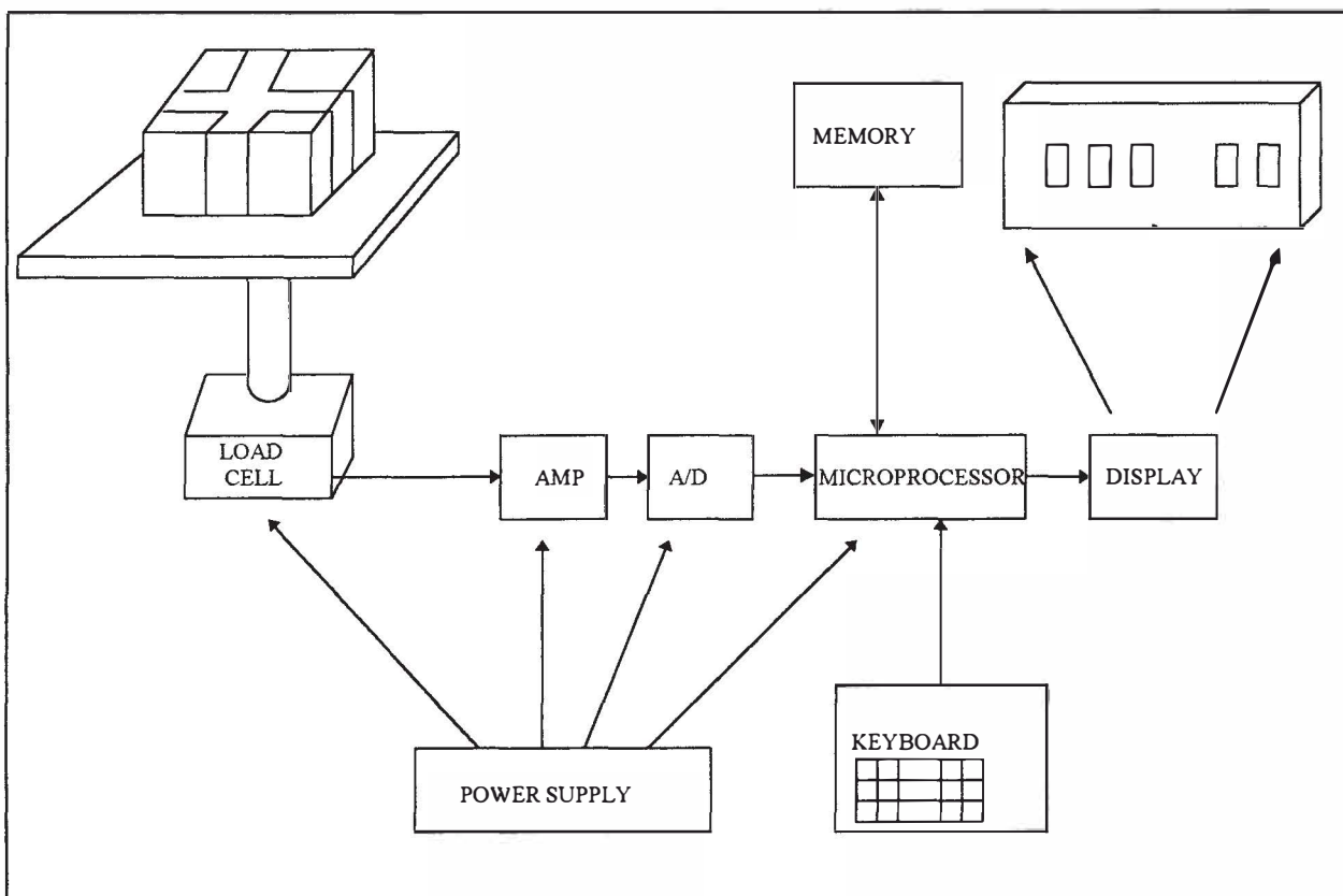
Figure 2: Block diagram of microcomputer-based smart scale
