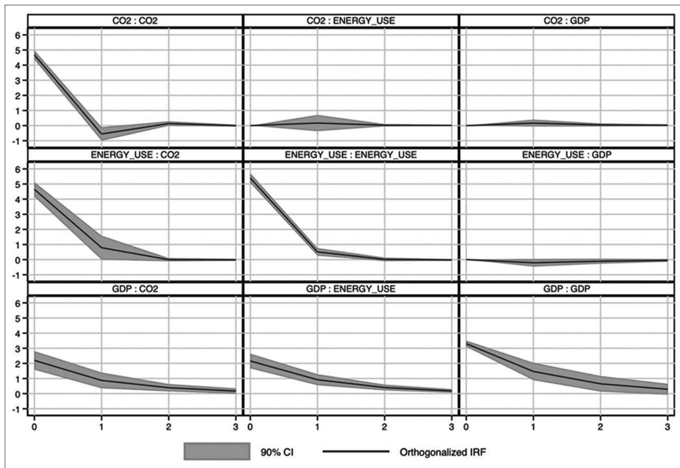
Figure 1: Impulse response analysis
