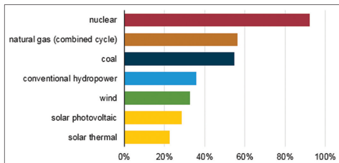
Figure 6: Capacity factors of selected generating technologies (US Energy Information Administration (EIA), 2016)
