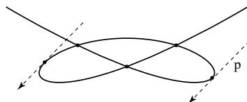
Figure 3.2: Critical points in X_s
