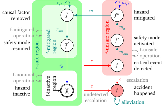
Figure 7: Refined notion of a risk factor f . The states of this LTS are called phases, the transitions are labelled with events and actions. Endangerment e (monitored) and accident e events; actions m_* and r_* of the safety controller with the actions m_{sf} and r_a where the controller interacts with the process waiting for a response; in gray, arbitrary process actions not controllable or observable by the safety controller.
