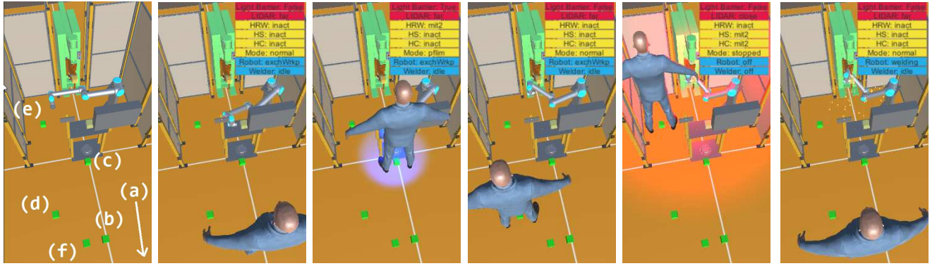
(a) System configuration for testing, with the operator's path highlighted by numbered waypoints. (b) Initial state. The operator waits in front of the workbench while the robot moves to retrieve a work piece. (c) The controller issues mitigations as the operator and robot simultaneously reach for the workbench ( HRW ). (d) The operator leaves the workbench while the robot in response to the operator approaches the spot welder. The risk factor has been removed. (e) The controller issues a stop in response to the operator approaching the spot welder during operation ( HS and HC ). (f) Welding resumes after operator leaves the work cell. The notification to leave the cell is deactivated.
