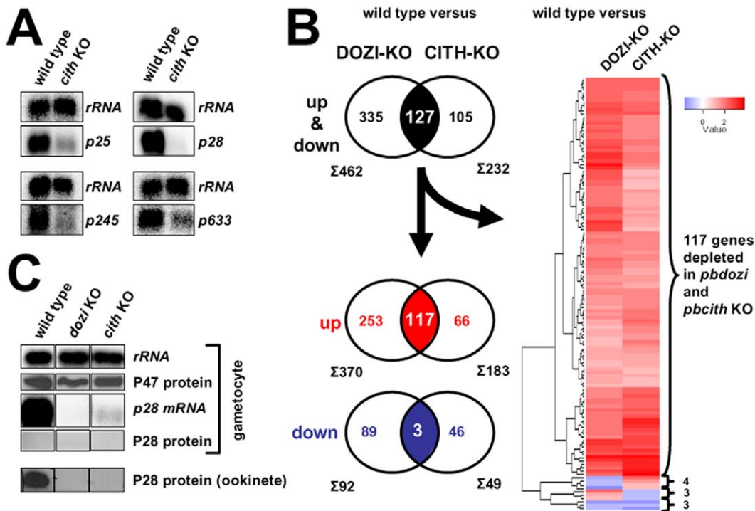
Figure 5. CITH and DOZI gene deletion mutant gametocytes suffer substantial mRNA loss. A Northern blot analysis of four translationally repressed transcripts in wild type and \Delta bcith mutants shows a clear de-stabilizing effect in the absence of CITH in gametocytes. B Venn diagrams of all 2-fold differentially expressed genes common to DOZI and CITH KO parasites. Hierarchical cluster analysis of the differentially expressed genes common to both lists. C Absence of DOZI or CITH does not result in the precocious translation of p28 mRNA into protein in female gametocytes. doi:10.1371/journal.ppat.1000767.g005
