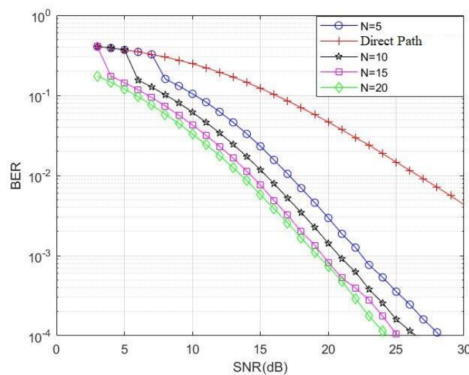
Figure 4.23. Multi-relay AF with Double-Threshold with P_s = 0.7P_t and P_r = 0.3P_t and Th_{In}=3 and Th_{Out}=5 for case(ii)
