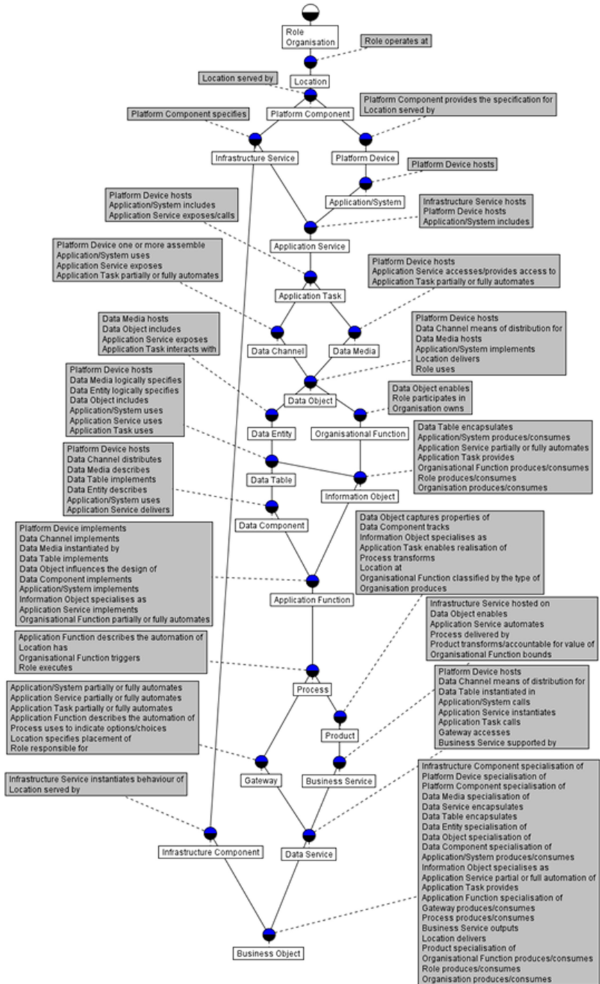
Fig. 4. 25v2ActiveInfrastructureService lattice
