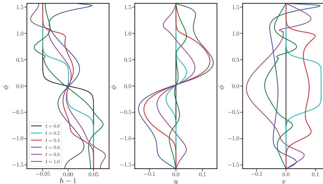
FIG. 2. Early time evolution of a dam-break initial condition for A=0.05 , w=0.1 and L_d=0.2 . The three panels show h-1 , u and v (left to right) at selected times as indicated. Note \phi is plotted on the ordinate. Numerically, n=500 intervals were used, with a time step \Delta t = 0.1\Delta a/c = 1/(40nL_d) = 1/4000 .
