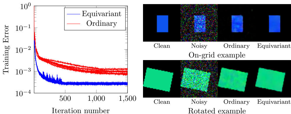
FIGURE 3. A demonstration of the use of equivariance in a denoising task. On the left, we have plotted training errors for 5 runs of each denoiser. On the right, we have displayed the outputs of the denoisers on an example (the "on-grid" example) similar to the ones used for training and on a rotated version.
