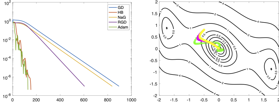
FIGURE 4. Optimisation of V(x, y) = 2x^2 - 1.05x^4 + 1/6x^6 + xy + y^2 . Comparison of gradient descent, Hamiltonian descent and Adam iterations, initial guess [-0.5, 0.8] , global minimum at [0, 0] . Methods and parameters: Gradient descent (GD) learning rate h = 0.01 , Heavy ball (HB) \mu = 0.9 , h = 0.01 , Nesterov Accelerated Gradient (NaG) \mu = 0.012 , h = 0.01 , Relativistic Gradient Descent (RGD) [49] h = 0.0001 , \mu = 0.9259 , Adam \beta_1 = 0.9 , \beta_2 = 0.999 , \varepsilon = 1e - 8 , \alpha = h = 0.1 . Left: value of the loss function versus number of iterations. Right: trajectory of approach to the optimum (NaG h = 0.01 yellow, RGD h = 0.0001 magenta, Adam h = 0.1 green).
