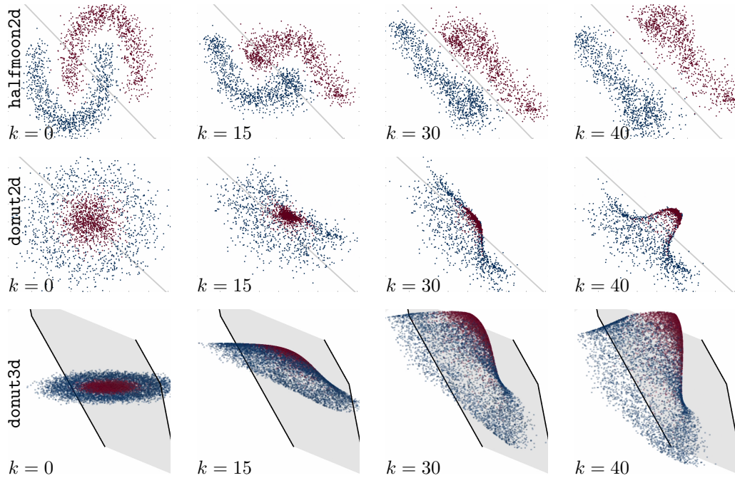
FIGURE 1. Evolutions of the ResNet model (6) for three different data sets. The upper two rows show evolutions in 2d and the lower row in 3d. The link function \sigma is the hyperbolic tangent and the data fit and regulariser are the squared 2-norm, L_n(z) = \frac{1}{2}\|z - y_n\|_2^2 , R(\theta) = \frac{\lambda}{2}\|\theta\|_2^2 .
