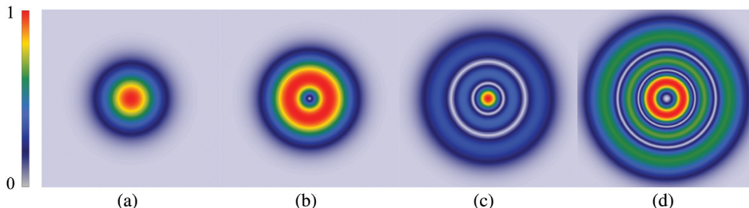
Fig. 4 Transverse intensity profiles of LG modes with (a) \text{LG}_0^0 , (b) \text{LG}_1^1 , (c) \text{LG}_2^0 , and (d) \text{LG}_2^2 . The color denotes the normalized intensity distribution.
