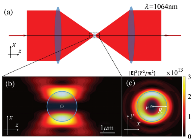
Fig. 41 Trapping of nanodiamonds with linearly polarized \text{LG}_{03} beams. (a) Schematic of the dual beam trap. (b) Geometry of the trap relative to a nanodiamonds-core (core radius r = 100 \text{ nm} ) coated with a silica shell (shell radius R = 1 \mu\text{m} ) (b) from the side and (c) axial views, respectively. Adapted from Ref. 112.
