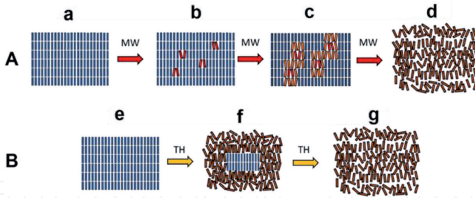
Figure 5. A: Proposed (a, b, c and d) microwave (MW) heating processes within the liquid crystalline state. A small fraction of the liquid crystalline domain (hot spots) changes to the isotropic phase during microwave irradiation. The rate of temperature increase in this isotropic phase domain is higher than that in the liquid crystalline phase because of the larger dielectric loss for the isotropic phase. B: Schematic diagram showing the thermal heating process (e, f, and g) starting from the liquid crystalline phase to the isotropic phase [33].
