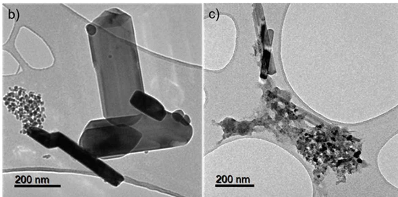
Fig. 1 (a) XRD patterns (Mo-K \alpha radiation) of the V 2 O 5 and V 2 O 5 -TiO 2 materials, with an \alpha -V 2 O 5 reference pattern (PDF 01-072-0433). TiO 2 diffraction peaks are indicated with asterisks (*), and the minor impurity peaks assigned to V 6 O 11 indicated with ●; (b) TEM images of V 2 O 5 ; (c) TEM images of V 2 O 5 -TiO 2 .
