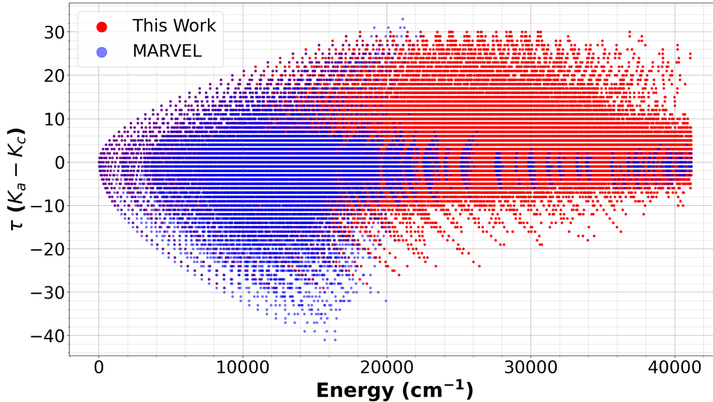
Figure 2: Our calculated states with \sum_{\alpha\beta\gamma}(\Psi_{\alpha\beta\gamma}^{J,k})^2 > 0.5 and MARVEL [17] states superimposed.
