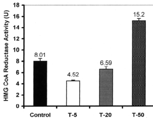
Figure 3. Effect of \alpha -tocopherol (T) on HMG CoA reductase activity
