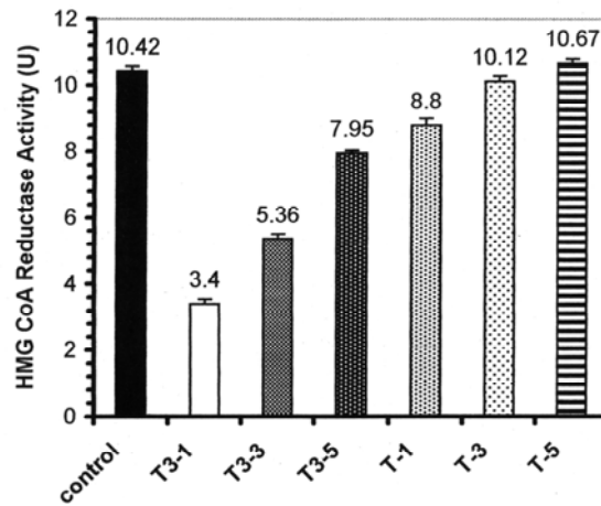
Figure 1. Effect of tocotrienols (T3) and \alpha -tocopherol (T) on HMG CoA reductase activity
