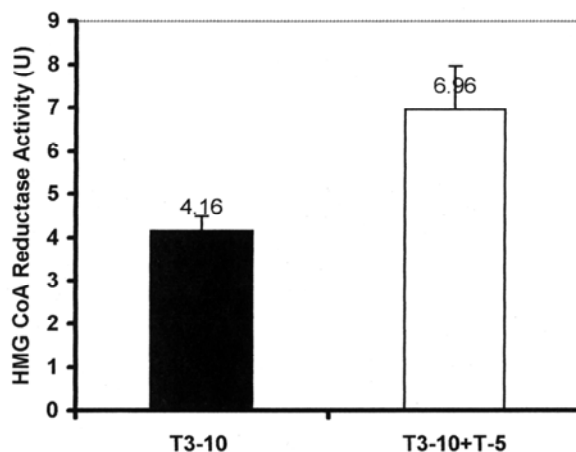
Figure 4. \alpha -Tocopherol (T) attenuates inhibitory activity of tocotrienols (T3) on HMG CoA reductase
