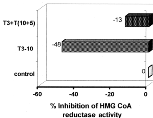
Figure 5. Percentage inhibition / activation of HMG CoA reductase activity by tocotrienols (T3) and a mixture of tocotrienols (T3) and \alpha -tocopherol (T)
