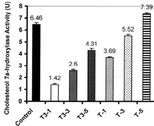
Figure 6. Effect of tocotrienols (T3) and α-tocopherol (T) on cholesterol 7 α-hydroxylase activity
