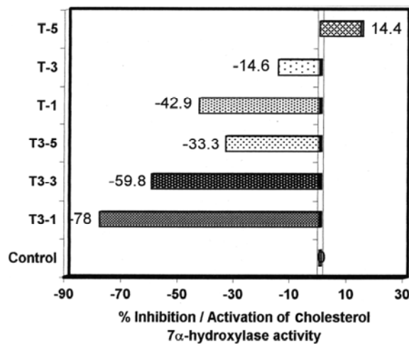
Figure 7. Percentage inhibition / activation of cholesterol 7 α-hydroxylase activity by tocotrienols (T3) and α-tocopherol (T)
