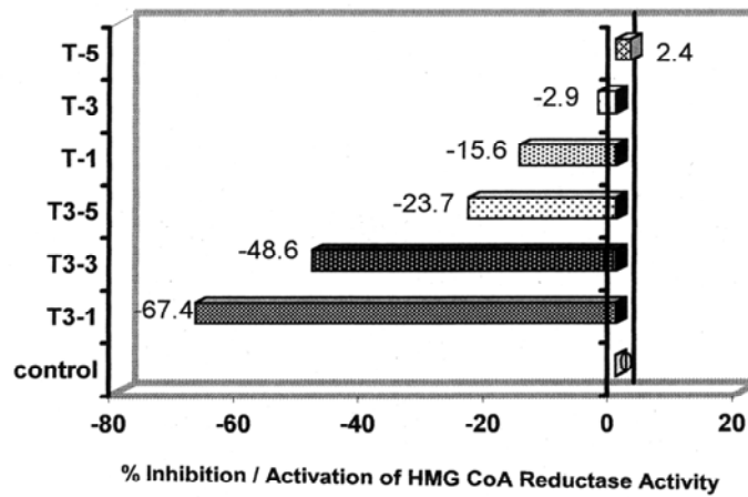
Figure 2. Percentage inhibition / activation of HMG CoA reductase by tocotrienols (T3) and \alpha -tocopherol (T)
