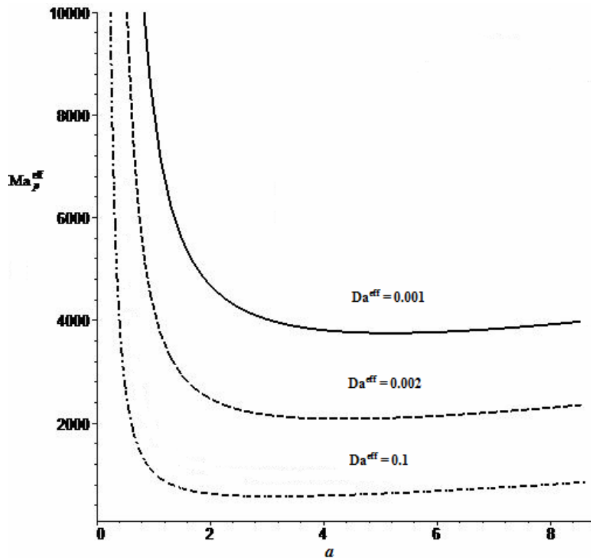
Figure 3: Variation of Ma_p^{\text{eff}} with a for different values of Da^{\text{eff}} in the case Bi = 2 .
