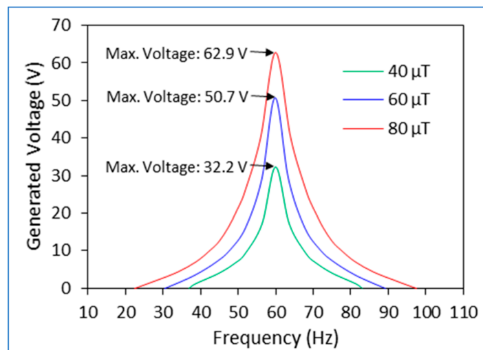
Figure 3. Finite element results of the maximum voltages according to the variations of magnetic field and frequency.
