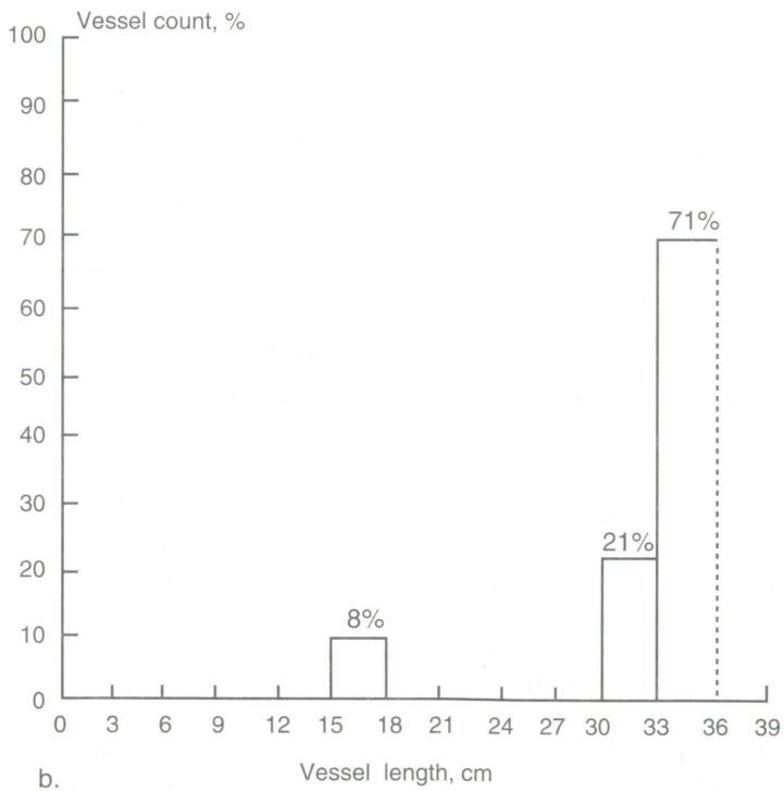
Fig 2. a: A count of vessels that are cut open at both ends, follows the line A-B-C-D-E; b: The resulting bar diagram shows vessel length distribution
