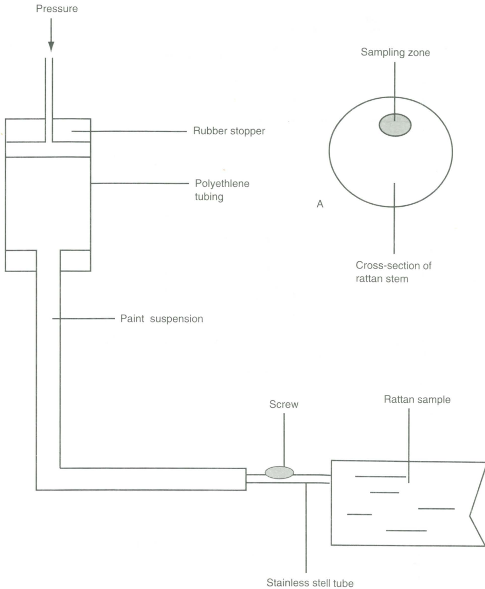
Fig. 1. Schematic diagram of the apparatus used to infuse alkyd-paint into a rattan sample. A: The paint applicator is tapped into the shaved end near the periphery of the rattan stem for random sampling
