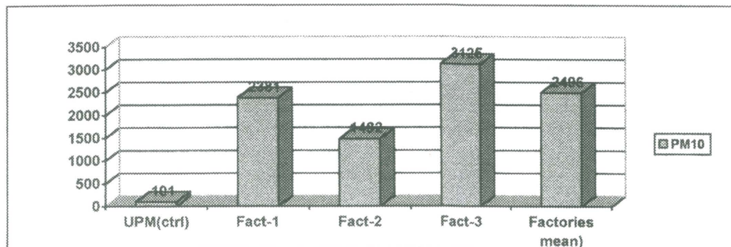
Fig. 1. Mean PM 10 concentration in the control and study areas
