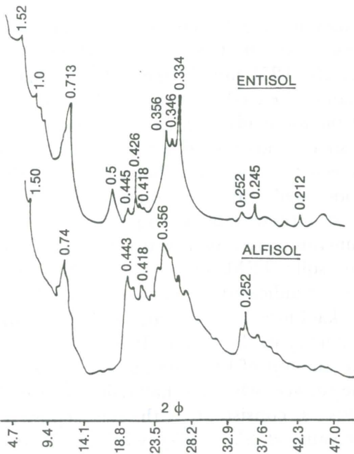
Fig. 1 X-ray diffraction patterns of Mg-saturated clay fraction from the A horizon of the Entisol and Alfisol.
