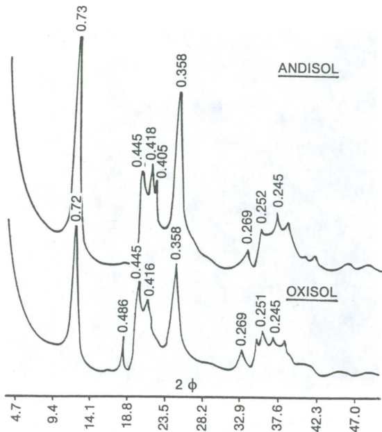
Fig. 2 X-ray diffraction patterns of Mg-saturated clay fraction from the A horizon of the Andisol and Oxisol
