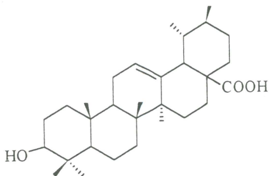
(II) ursolic acid
