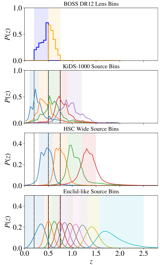
Figure 8. Redshift distributions P(z) for the lens and source galaxy samples used in the forecasts for the galaxy-galaxy lensing signal in a KiDS-1000+BOSS, HSC Wide+BOSS and Euclid -like+DESI-like analysis. The properties of these redshift distributions are given in table 2. The black vertical dot-dashed lines show the limits of the BOSS lens bins for comparison with the source bins.
