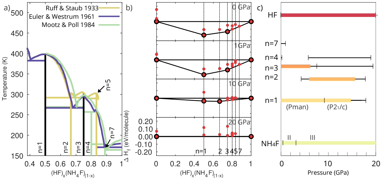
FIG. 6. Ground state energetics of the \text{NH}_4\text{F} – \text{HF} system. a) Experimental composition phase diagrams adapted from 68–70 . Black lines mark phases seen in all experiments, to the highest measured melt temperature. Solid compositions \text{NH}_4\text{F}(\text{HF})_n include n = 1 - 5 and 7. b) Calculated convex hulls of relative formation enthalpies of \text{NH}_4\text{F} – \text{HF} compounds. The structures are of the form (\text{NH}_4)^+(\text{H}_n\text{F}_{n+1})^- where n is given along vertical dashed lines. c) Calculated ground state phase diagram as a function of pressure. Stable phases are coloured lines and metastable phases (less than 10 meV removed from the convex hull) are thin black lines.
