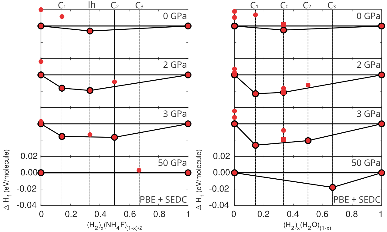
FIG. 4. Relative formation enthalpies for mixtures in the binary systems \text{NH}_4\text{F}-\text{H}_2 (left) and \text{H}_2\text{O}-\text{H}_2 (right), at a series of pressures. Solid black lines and outlined symbols denote convex hulls and calculated stable phases. Square symbols in the \text{H}_2\text{O}-\text{H}_2 panel represent \text{C}_0 .
