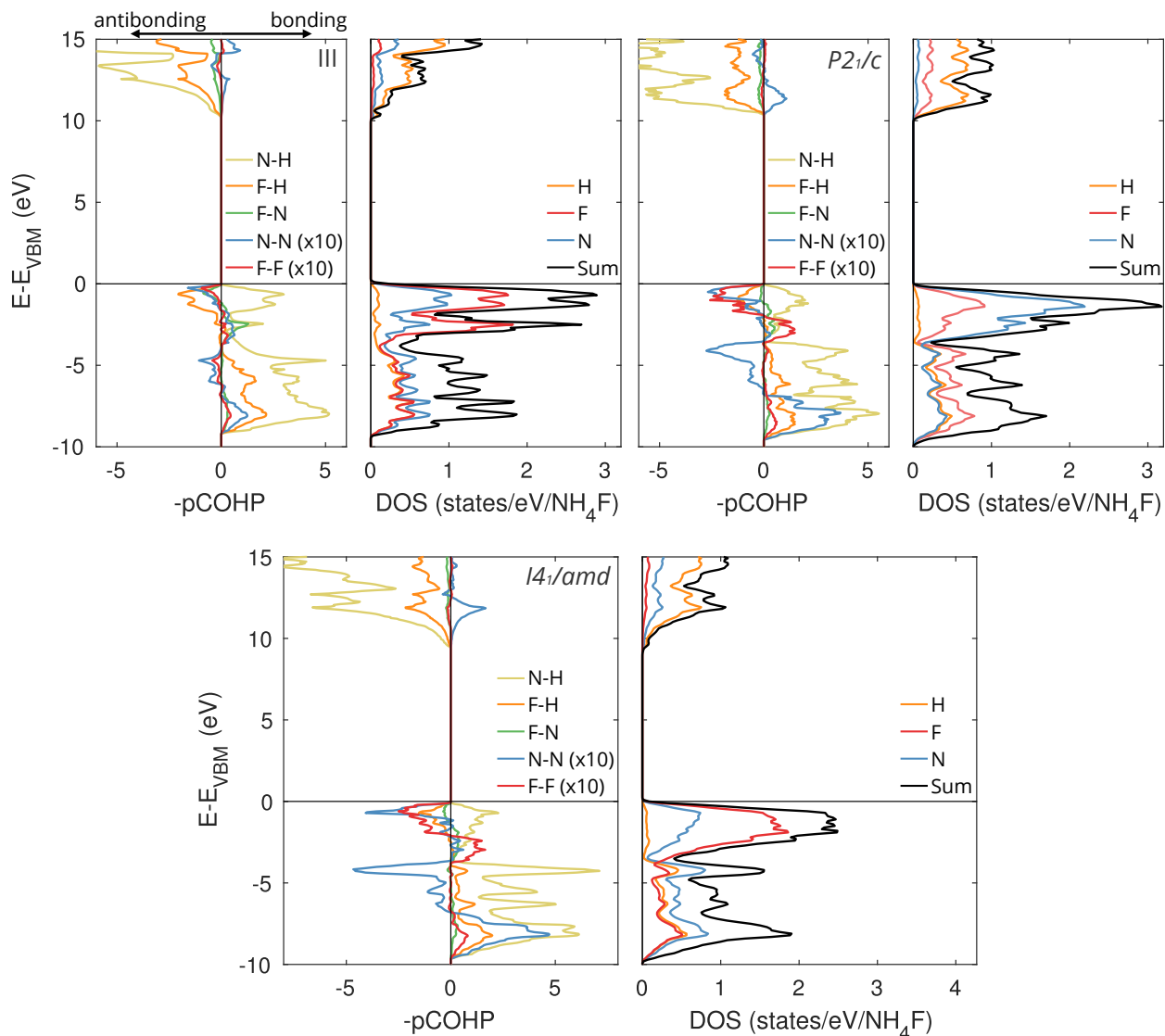
FIG. 3. Crystal orbital Hamilton populations (pCOHP) and partial density of states (pDOS) for the \text{NH}_4\text{F} structures at 100 GPa. pCOHP values are averaged over all first neighbour shells of each bond type and normalized per \text{NH}_4\text{F} formula unit. F-F and N-N populations are enhanced by a factor of 10 for clarity.
