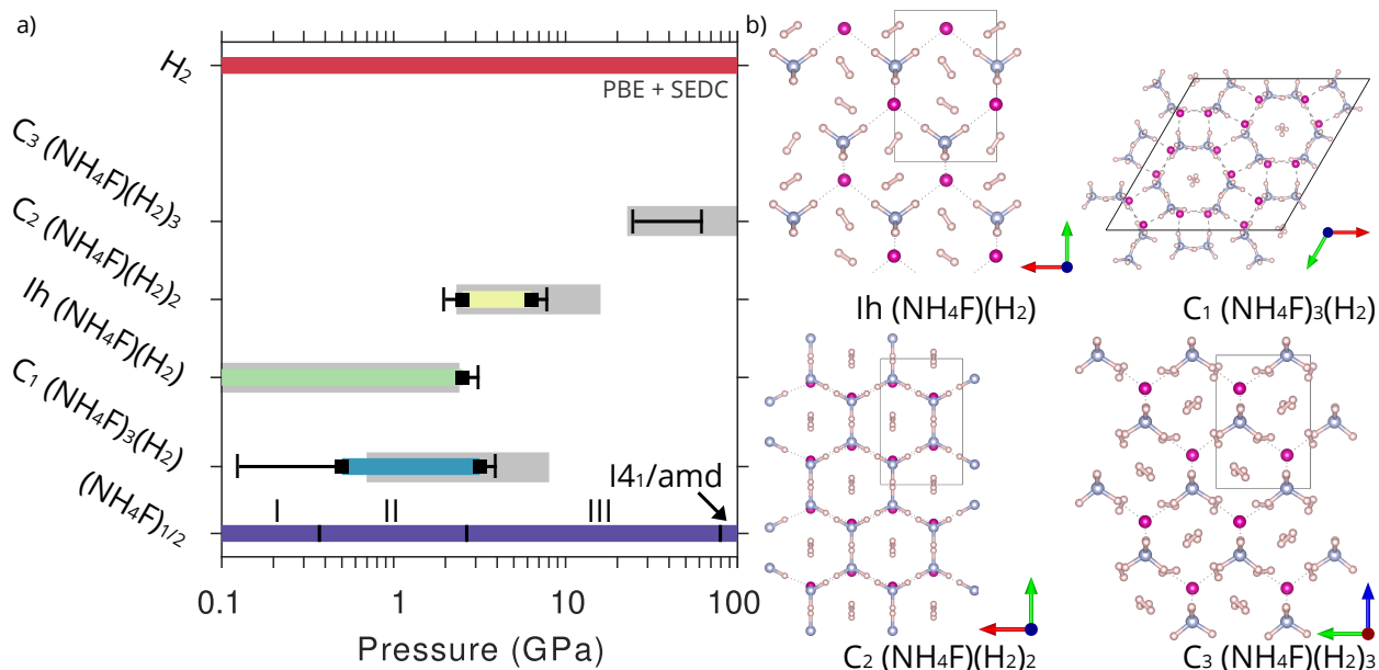
FIG. 5. a) Ground-state phase diagram for the \text{NH}_4\text{F}-\text{H}_2 binary system as function of pressure and composition. Colored bars indicate pressure regions of stability. Black lines indicate metastability (see main text). Grey bars represent the corresponding stability regions calculated for the \text{H}_2\text{O}-\text{H}_2 analogues. b) Unit cells for structures. \text{C}_1 is shown in a conventional unit cell setting.
