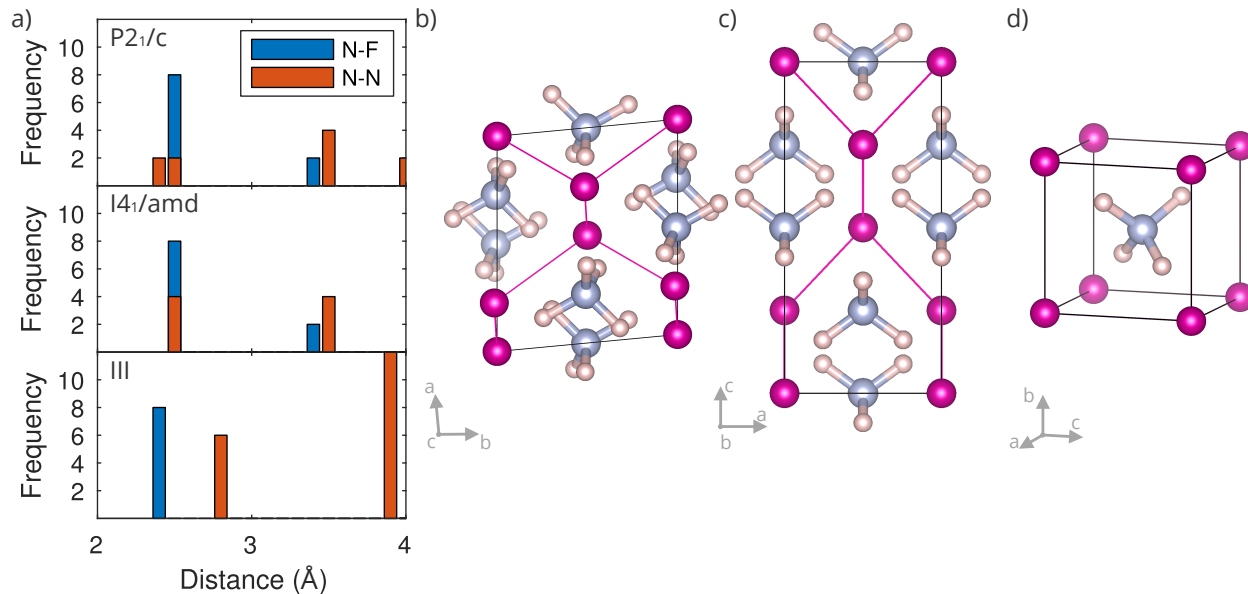
FIG. 2. a) Pair distribution functions for the heavy atom lattices at 100 GPa. Crystal structures of (b) \text{NH}_4\text{F} - P2_1/c , (c) I4_1/amd , and (d) III at 100 GPa. F–F nearest neighbours are connected as a guide to the eye.
