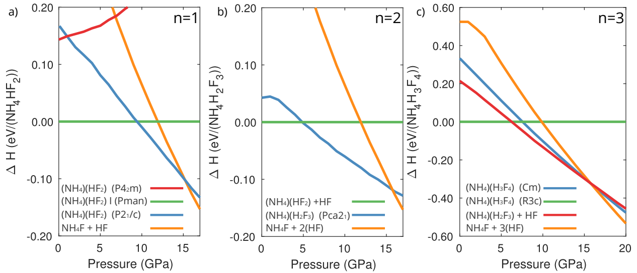
FIG. 7. Enthalpy values as a function of pressure for the \text{NH}_4\text{F}(\text{H}_n\text{F}_{n+1}) compounds a) (\text{NH}_4\text{F})^+(\text{HF}_2)^- , b) (\text{NH}_4\text{F})(\text{H}_2\text{F}_3) , c) (\text{NH}_4\text{F})(\text{H}_3\text{F}_4) .
