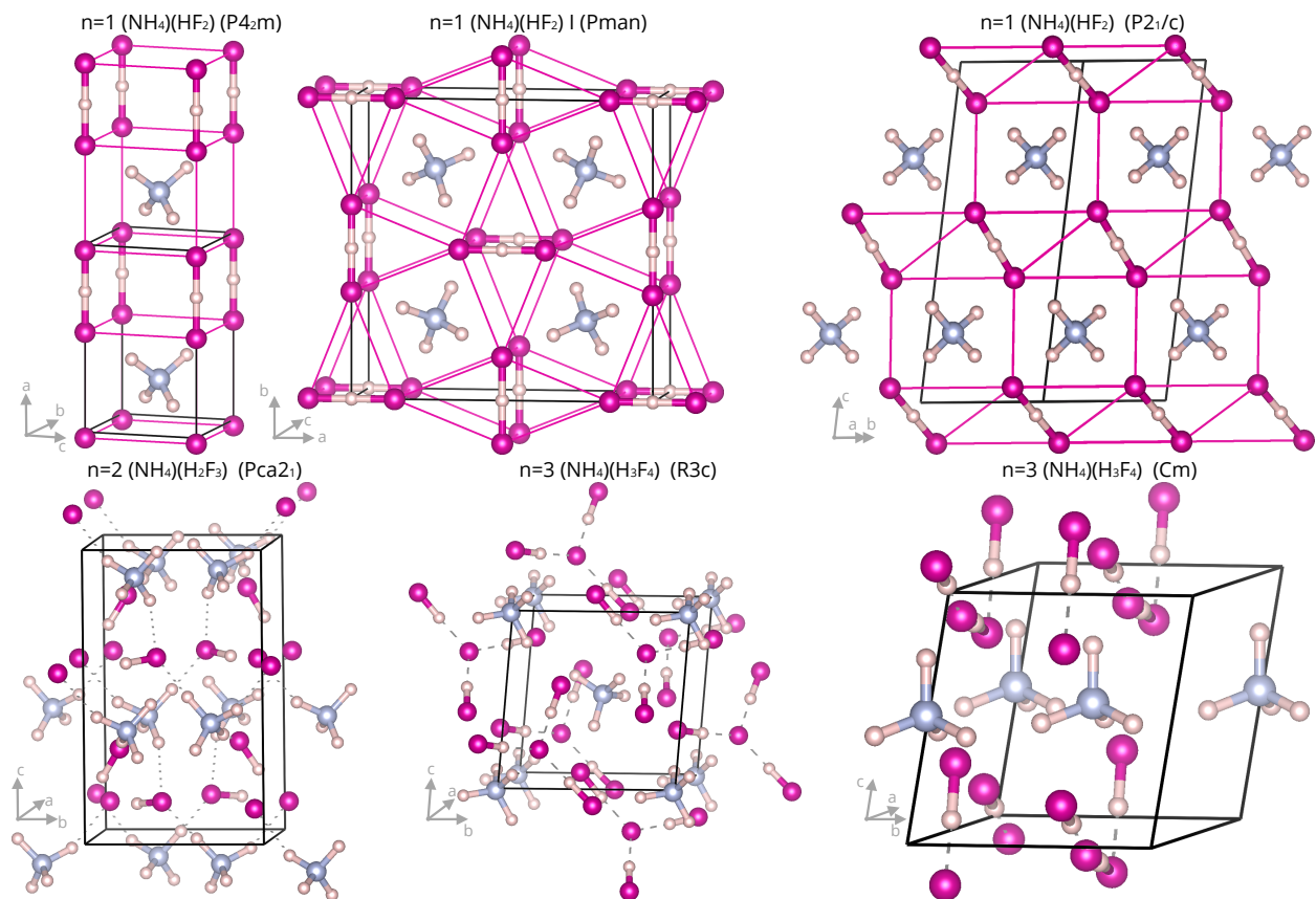
FIG. 8. Crystal structures for HF-rich mixtures \text{NH}_4\text{F}(\text{HF})_n , labelled by n and space group. Some structural motifs highlighted by thin pink lines connection neighbouring fluorine atoms.
