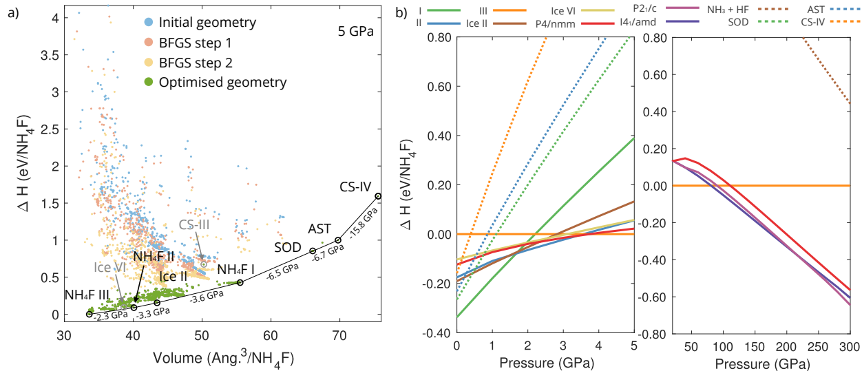
FIG. 1. a) Enthalpy-volume scatter plot of \text{NH}_4\text{F} structures at 5 GPa resulting from the \text{H}_2\text{O} structures from Engel et al. 37 Data points relate to enthalpies and volumes for initial geometries (blue), the first two optimisation steps (red, yellow), and the optimised geometries (green). Black circles represent the convex hull, with structure types labeled. Gradients of the connections between these structures represent the transition pressures, relative to 5 GPa. Grey circles and labels highlight other water ice geometries. b) Relative enthalpies as a function of pressure, in a low pressure (up to 5 GPa) and high pressure regime (up to 300 GPa).
