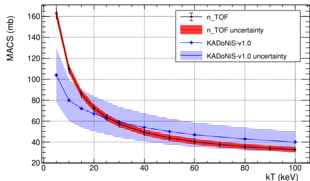
FIG. 4. Maxwellian-averaged cross sections of this work (n_TOF) from kT = 5 to 100 keV compared to MACS values recommended in the latest version of the database KADoNiS-v1.0 [16].
