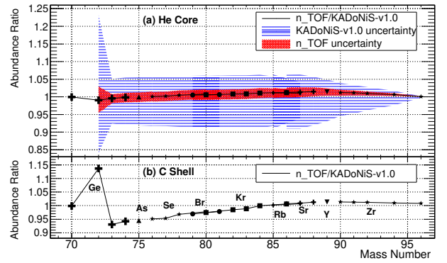
FIG. 5. Abundances produced in the s -process for a 25 solar mass star using the new cross sections determined at n_TOF. Abundances are normalised to results using the ^{72}\text{Ge}(n, \gamma) MACSs recommended in KADoNiS-v1.0 [16]. Isotopes of the same elements are connected by thin solid lines. Panel (a) shows abundances after He core burning. The shaded areas represent abundance variations when taking into account uncertainties of KADoNiS (blue) or n_TOF (red) cross sections. Panel (b) shows abundances after the later C shell burning phase.
